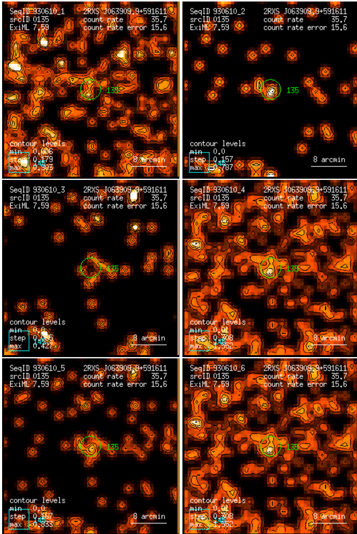
Figure 135: RASS 930610: detection 0135: band rate images, Gaussian filter: (1) PSPC channels 11 – 41, (2) 52 – 90, (3) 91 – 201, (4) 11 – 235, (5) 52 – 201, (6) 11 – 201. Broad band rates in counts/ks. Band rate contour levels in counts/ks/arcmin 2 .
