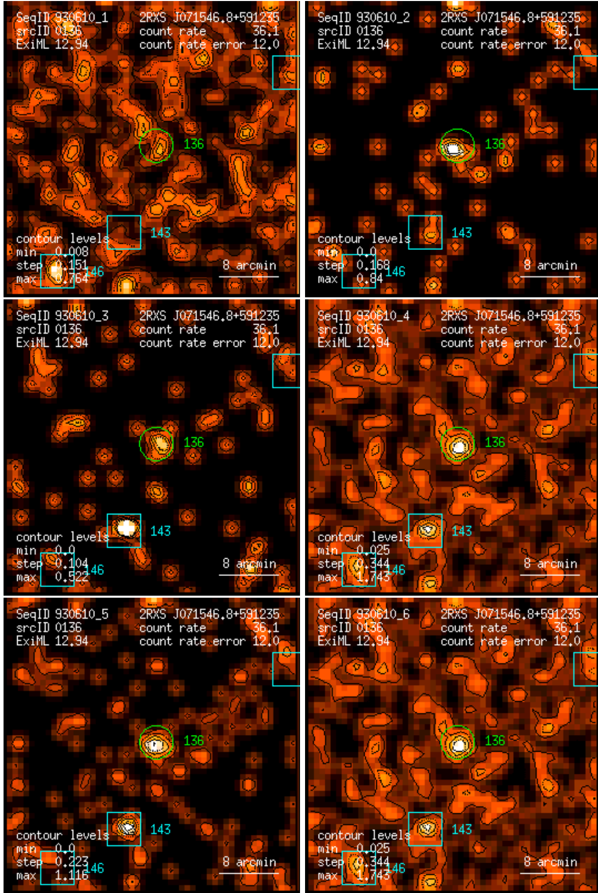
Figure 136: RASS 930610: detection 0136: band rate images, Gaussian filter: (1) PSPC channels 11 – 41, (2) 52 – 90, (3) 91 – 201, (4) 11 – 235, (5) 52 – 201, (6) 11 – 201. Broad band rates in counts/ks. Band rate contour levels in counts/ks/arcmin 2 .
