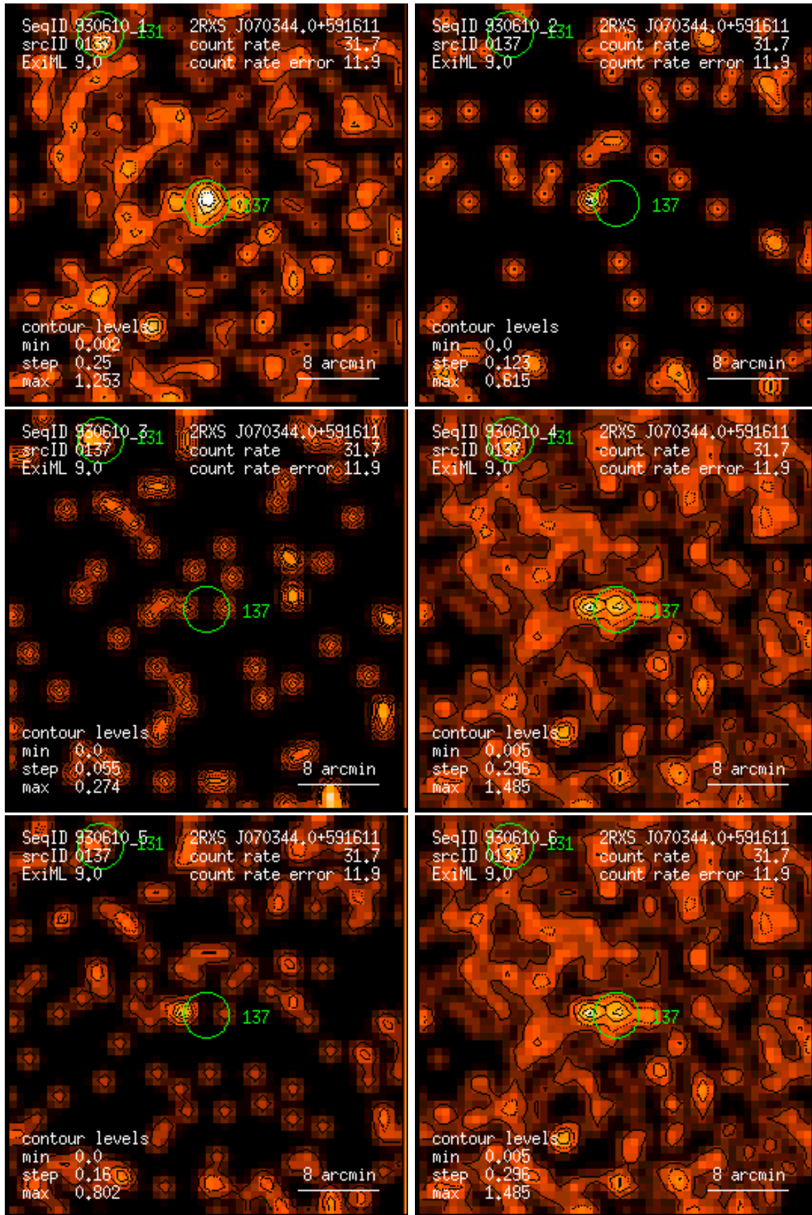
Figure 137: RASS 930610: detection 0137: band rate images, Gaussian filter: (1) PSPC channels 11 – 41, (2) 52 – 90, (3) 91 – 201, (4) 11 – 235, (5) 52 – 201, (6) 11 – 201. Broad band rates in counts/ks. Band rate contour levels in counts/ks/arcmin 2 .
