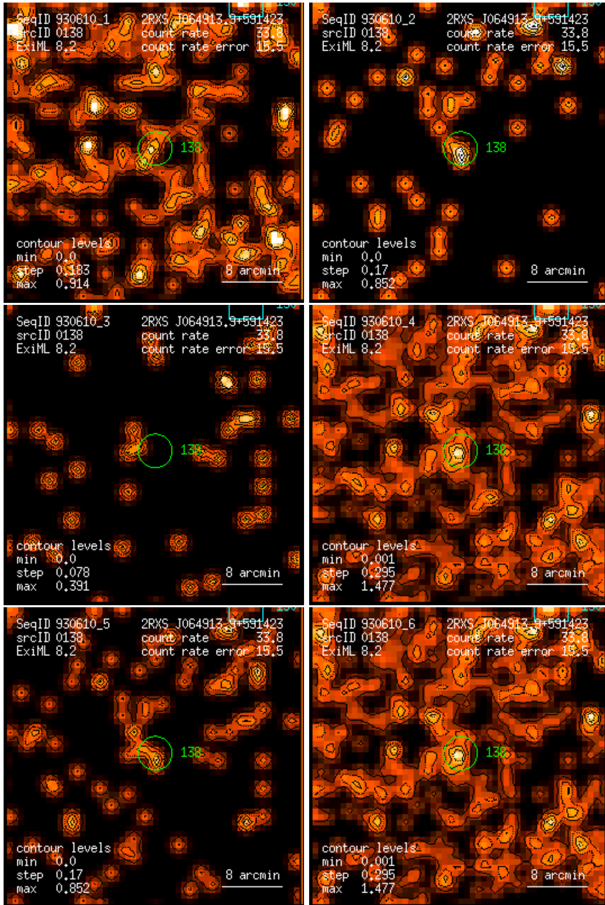
Figure 138: RASS 930610: detection 0138: band rate images, Gaussian filter: (1) PSPC channels 11 – 41, (2) 52 – 90, (3) 91 – 201, (4) 11 – 235, (5) 52 – 201, (6) 11 – 201. Broad band rates in counts/ks. Band rate contour levels in counts/ks/arcmin 2 .
