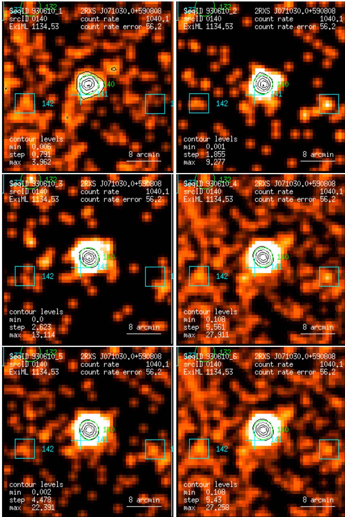
Figure 140: RASS 930610: detection 0140: band rate images, Gaussian filter: (1) PSPC channels 11 – 41, (2) 52 – 90, (3) 91 – 201, (4) 11 – 235, (5) 52 – 201, (6) 11 – 201. Broad band rates in counts/ks. Band rate contour levels in counts/ks/arcmin 2 .
