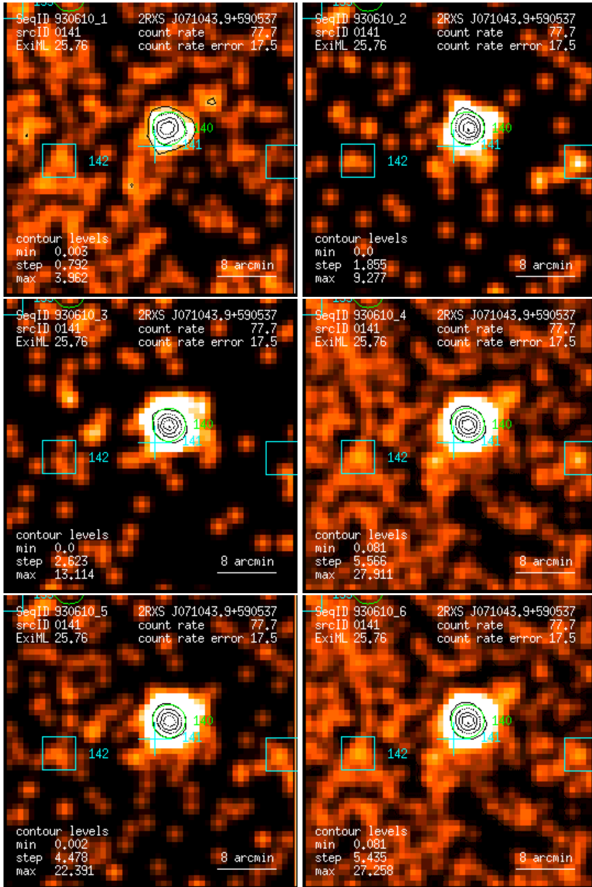
Figure 141: RASS 930610: detection 0141: band rate images, Gaussian filter: (1) PSPC channels 11 – 41, (2) 52 – 90, (3) 91 – 201, (4) 11 – 235, (5) 52 – 201, (6) 11 – 201. Broad band rates in counts/ks. Band rate contour levels in counts/ks/arcmin 2 .
