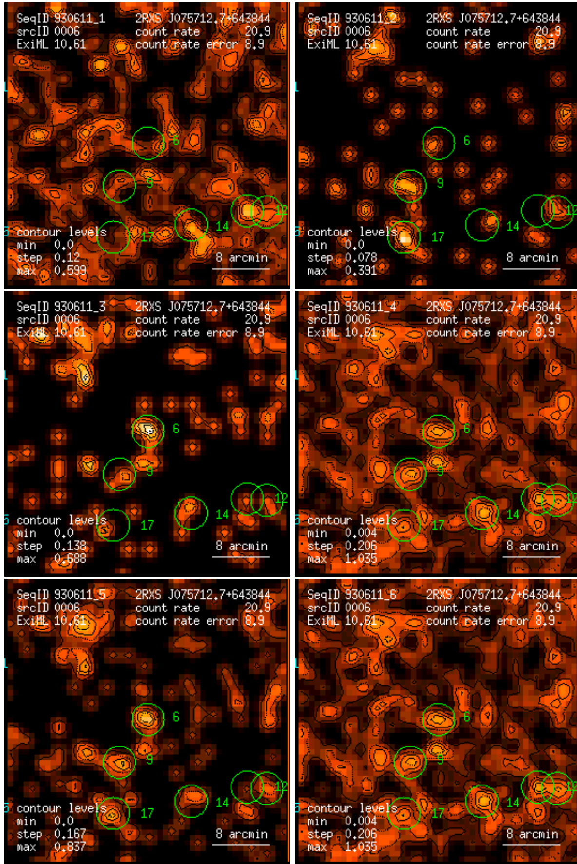
Figure 6: RASS 930611: detection 0006: band rate images, Gaussian filter: (1) PSPC channels 11 – 41, (2) 52 – 90, (3) 91 – 201, (4) 11 – 235, (5) 52 – 201, (6) 11 – 201. Broad band rates in counts/ks. Band rate contour levels in counts/ks/arcmin 2 .
