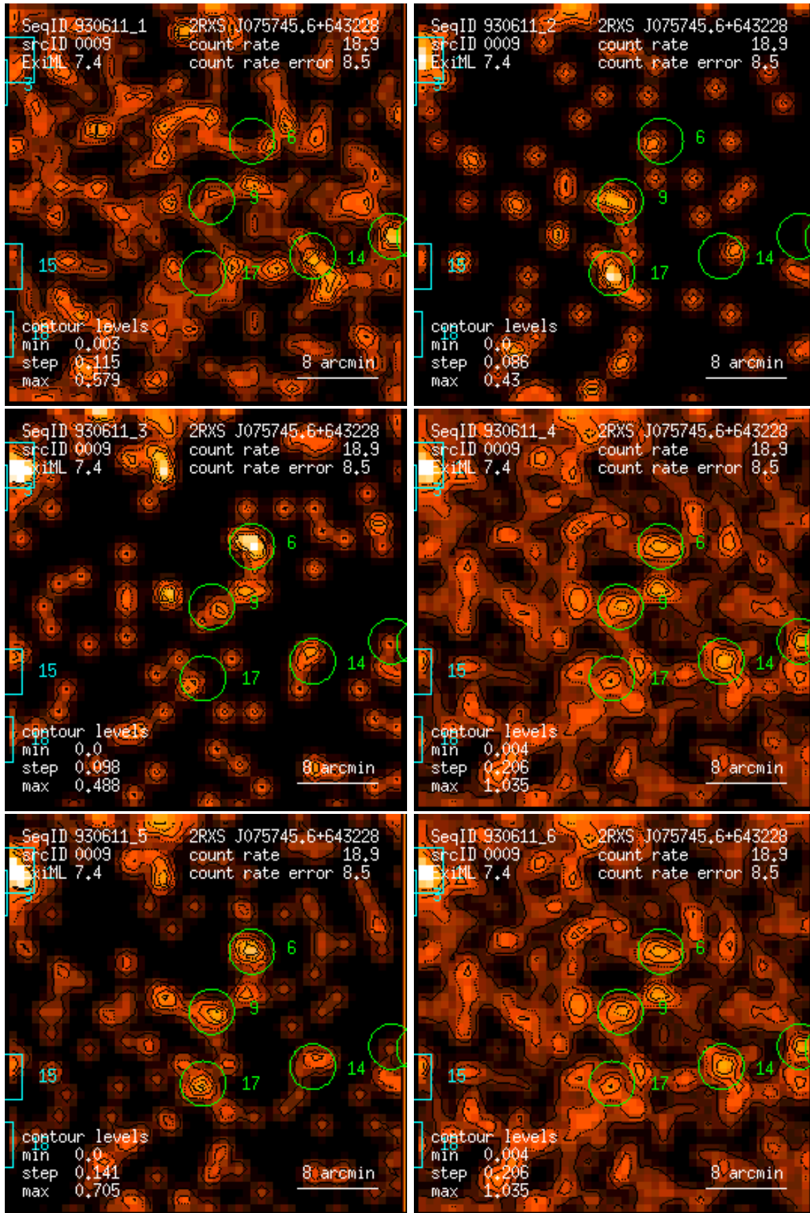
Figure 9: RASS 930611: detection 0009: band rate images, Gaussian filter: (1) PSPC channels 11 – 41, (2) 52 – 90, (3) 91 – 201, (4) 11 – 235, (5) 52 – 201, (6) 11 – 201. Broad band rates in counts/ks. Band rate contour levels in counts/ks/arcmin 2 .
