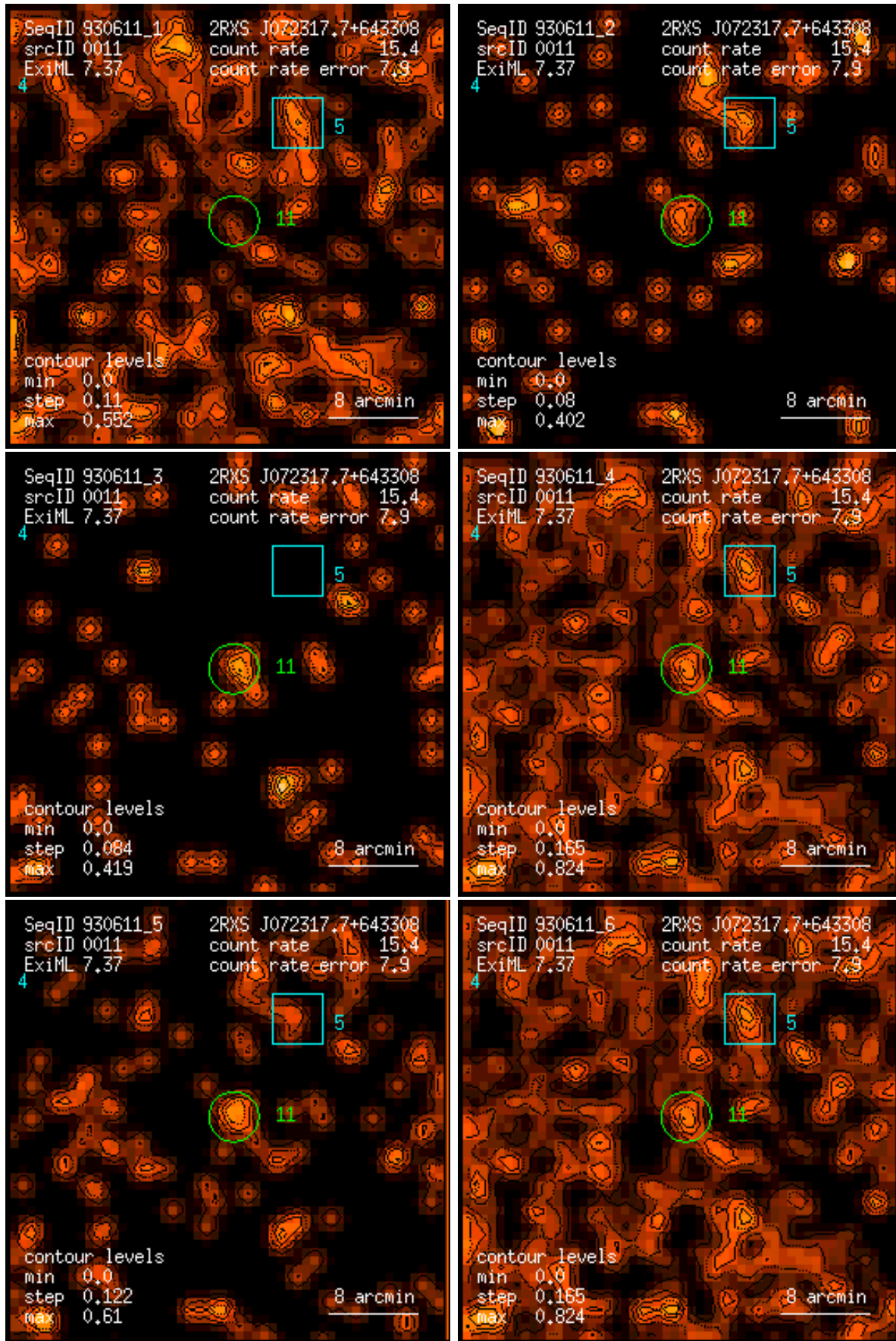
Figure 11: RASS 930611: detection 0011: band rate images, Gaussian filter: (1) PSPC channels 11 – 41, (2) 52 – 90, (3) 91 – 201, (4) 11 – 235, (5) 52 – 201, (6) 11 – 201. Broad band rates in counts/ks. Band rate contour levels in counts/ks/arcmin 2 .
