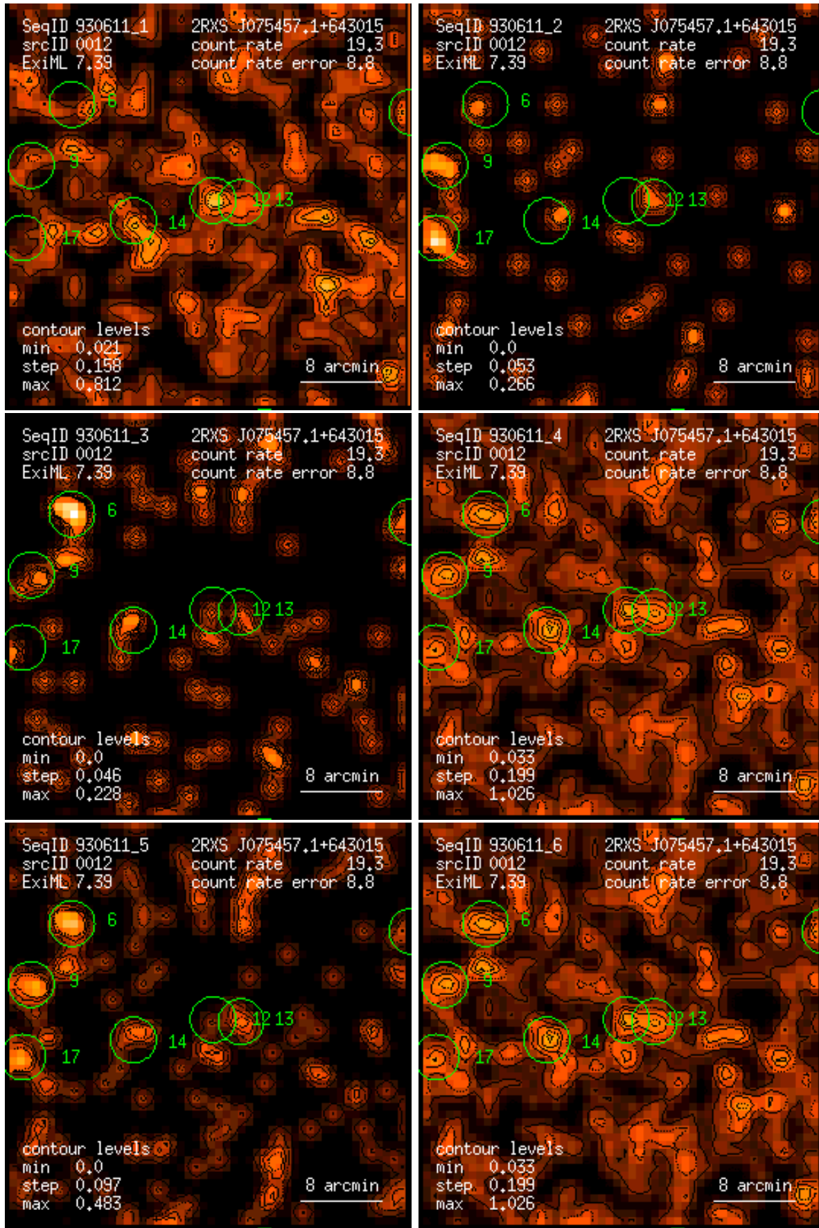
Figure 12: RASS 930611: detection 0012: band rate images, Gaussian filter: (1) PSPC channels 11 – 41, (2) 52 – 90, (3) 91 – 201, (4) 11 – 235, (5) 52 – 201, (6) 11 – 201. Broad band rates in counts/ks. Band rate contour levels in counts/ks/arcmin 2 .
