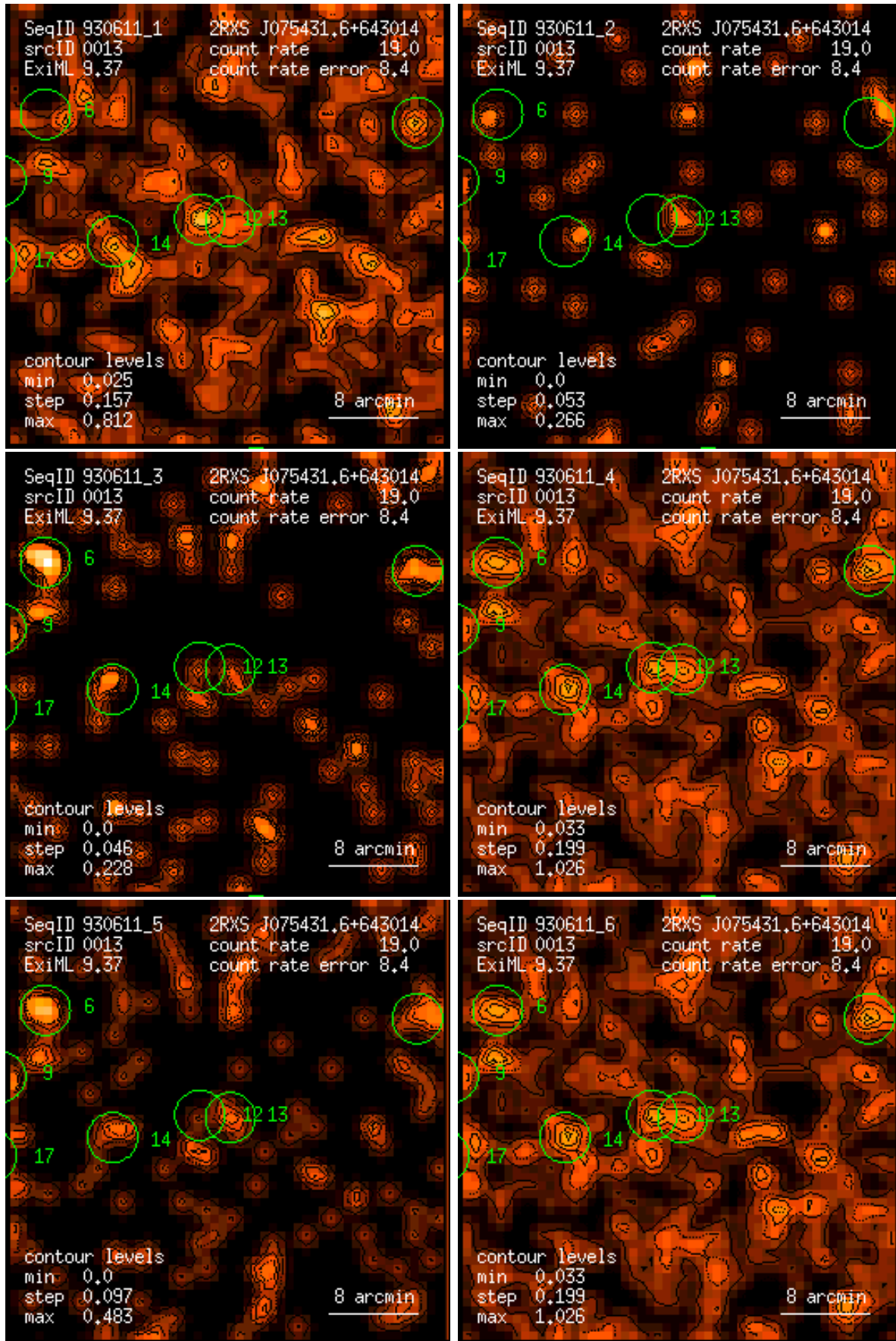
Figure 13: RASS 930611: detection 0013: band rate images, Gaussian filter: (1) PSPC channels 11 – 41, (2) 52 – 90, (3) 91 – 201, (4) 11 – 235, (5) 52 – 201, (6) 11 – 201. Broad band rates in counts/ks. Band rate contour levels in counts/ks/arcmin 2 .
