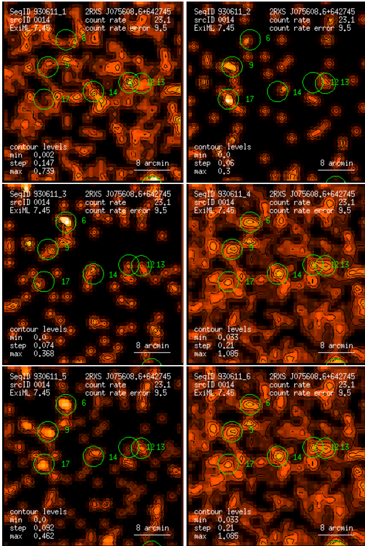
Figure 14: RASS 930611: detection 0014: band rate images, Gaussian filter: (1) PSPC channels 11 – 41, (2) 52 – 90, (3) 91 – 201, (4) 11 – 235, (5) 52 – 201, (6) 11 – 201. Broad band rates in counts/ks. Band rate contour levels in counts/ks/arcmin 2 .
