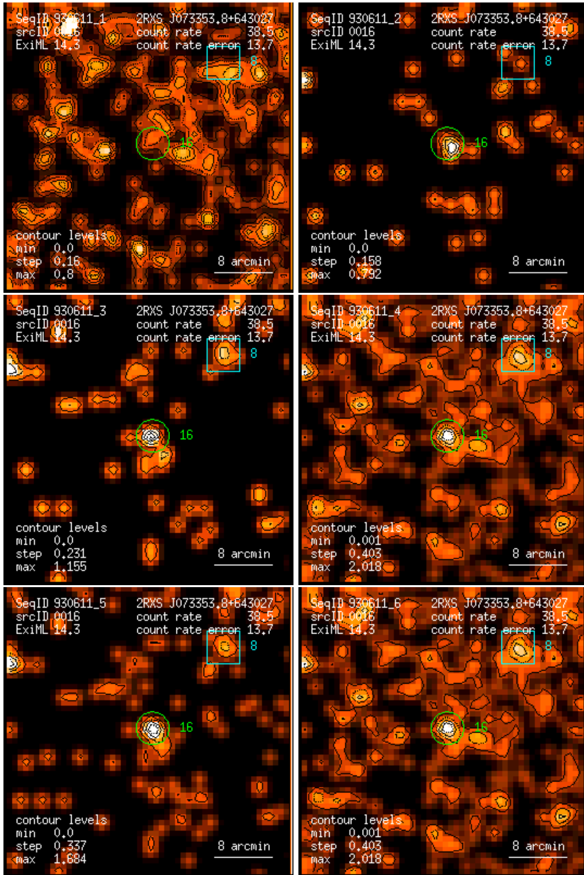
Figure 16: RASS 930611: detection 0016: band rate images, Gaussian filter: (1) PSPC channels 11 – 41, (2) 52 – 90, (3) 91 – 201, (4) 11 – 235, (5) 52 – 201, (6) 11 – 201. Broad band rates in counts/ks. Band rate contour levels in counts/ks/arcmin 2 .
