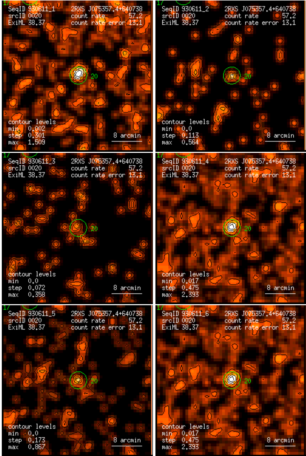
Figure 20: RASS 930611: detection 0020: band rate images, Gaussian filter: (1) PSPC channels 11 – 41, (2) 52 – 90, (3) 91 – 201, (4) 11 – 235, (5) 52 – 201, (6) 11 – 201. Broad band rates in counts/ks. Band rate contour levels in counts/ks/arcmin 2 .
