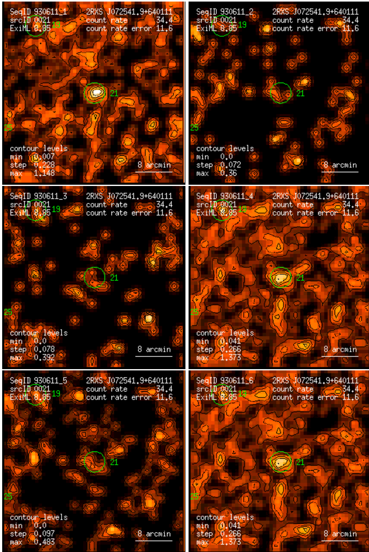
Figure 21: RASS 930611: detection 0021: band rate images, Gaussian filter: (1) PSPC channels 11 – 41, (2) 52 – 90, (3) 91 – 201, (4) 11 – 235, (5) 52 – 201, (6) 11 – 201. Broad band rates in counts/ks. Band rate contour levels in counts/ks/arcmin 2 .
