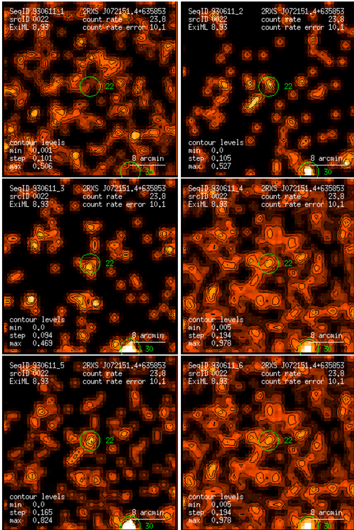
Figure 22: RASS 930611: detection 0022: band rate images, Gaussian filter: (1) PSPC channels 11 – 41, (2) 52 – 90, (3) 91 – 201, (4) 11 – 235, (5) 52 – 201, (6) 11 – 201. Broad band rates in counts/ks. Band rate contour levels in counts/ks/arcmin 2 .
