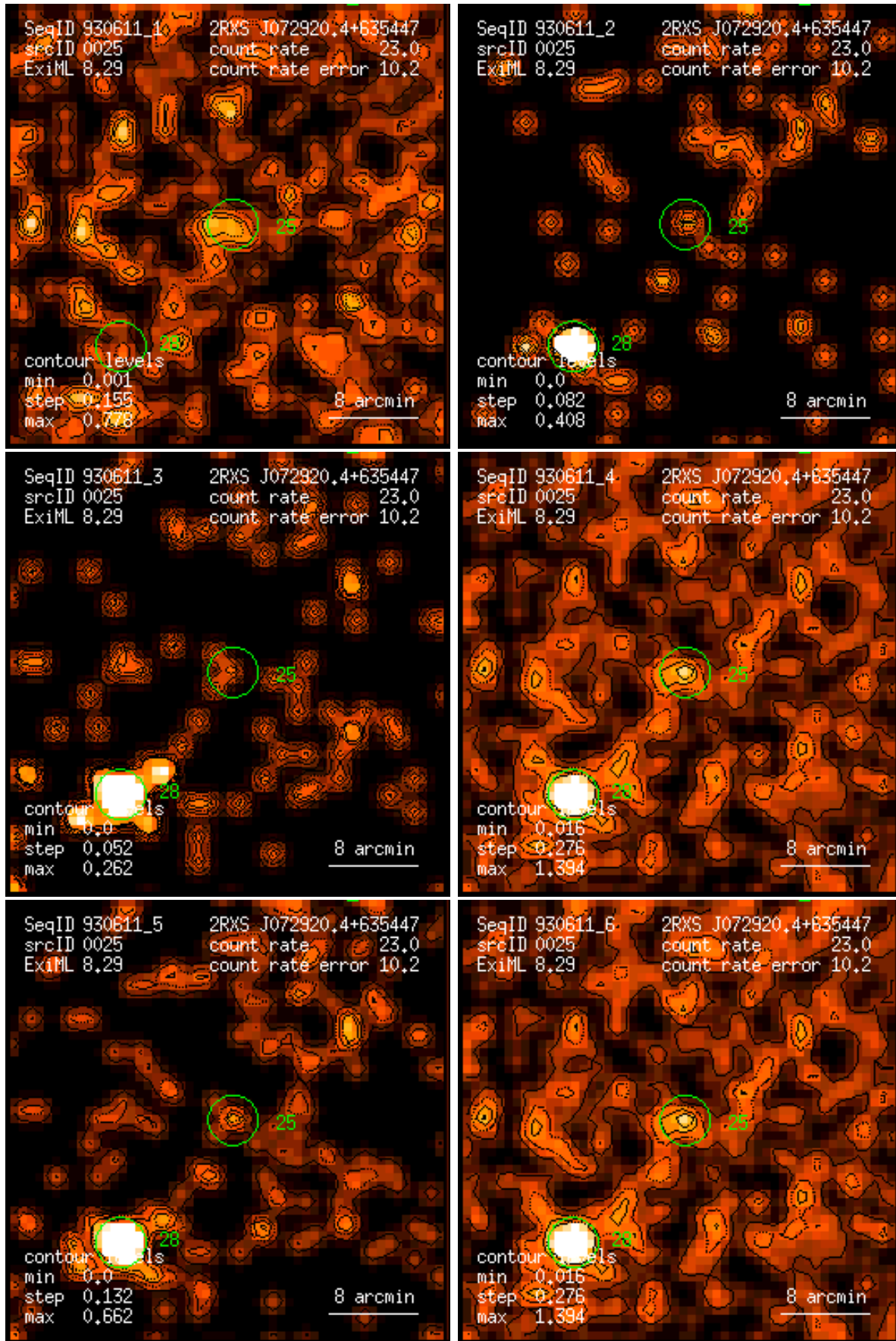
Figure 25: RASS 930611: detection 0025: band rate images, Gaussian filter: (1) PSPC channels 11 – 41, (2) 52 – 90, (3) 91 – 201, (4) 11 – 235, (5) 52 – 201, (6) 11 – 201. Broad band rates in counts/ks. Band rate contour levels in counts/ks/arcmin 2 .
