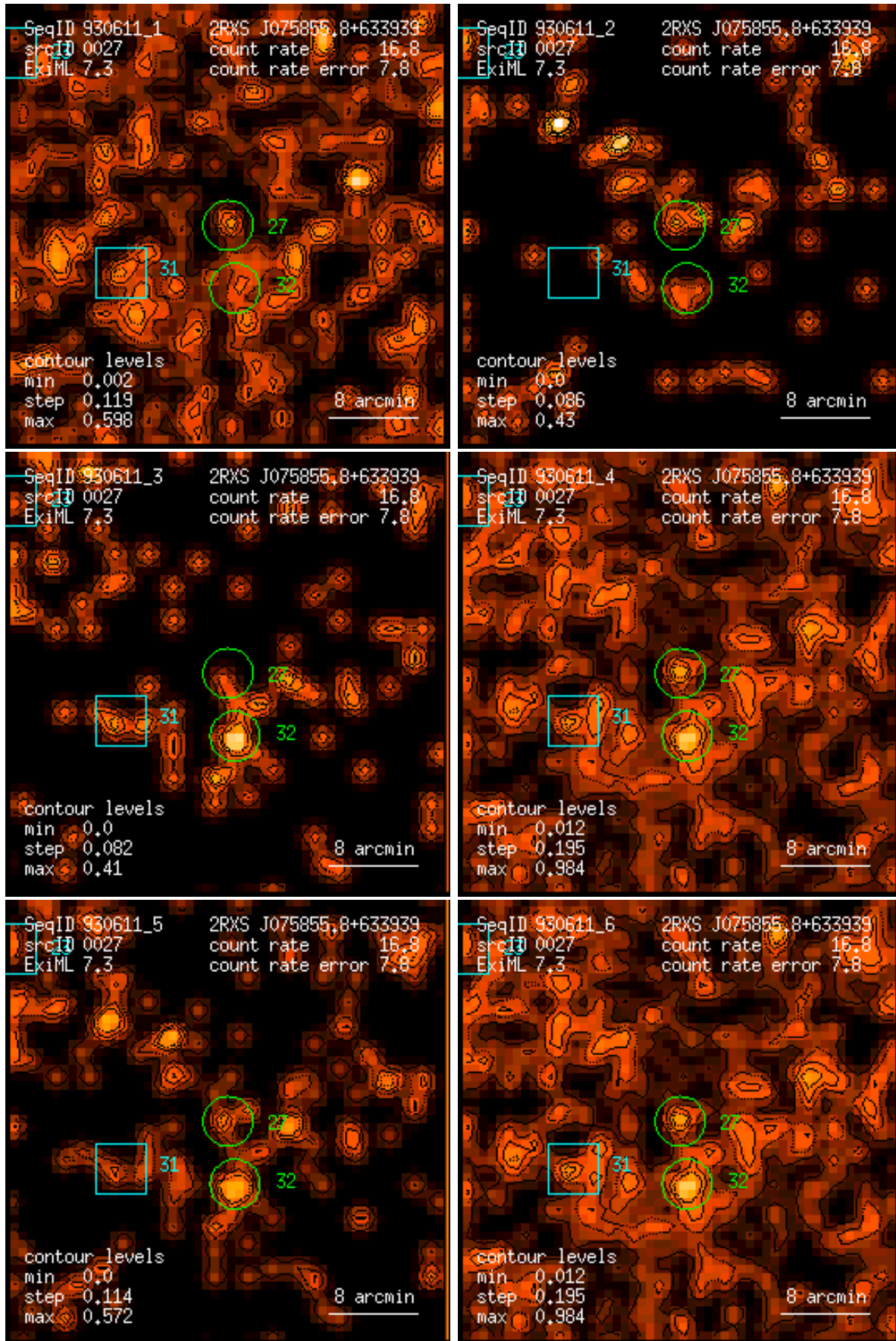
Figure 27: RASS 930611: detection 0027: band rate images, Gaussian filter: (1) PSPC channels 11 – 41, (2) 52 – 90, (3) 91 – 201, (4) 11 – 235, (5) 52 – 201, (6) 11 – 201. Broad band rates in counts/ks. Band rate contour levels in counts/ks/arcmin 2 .
