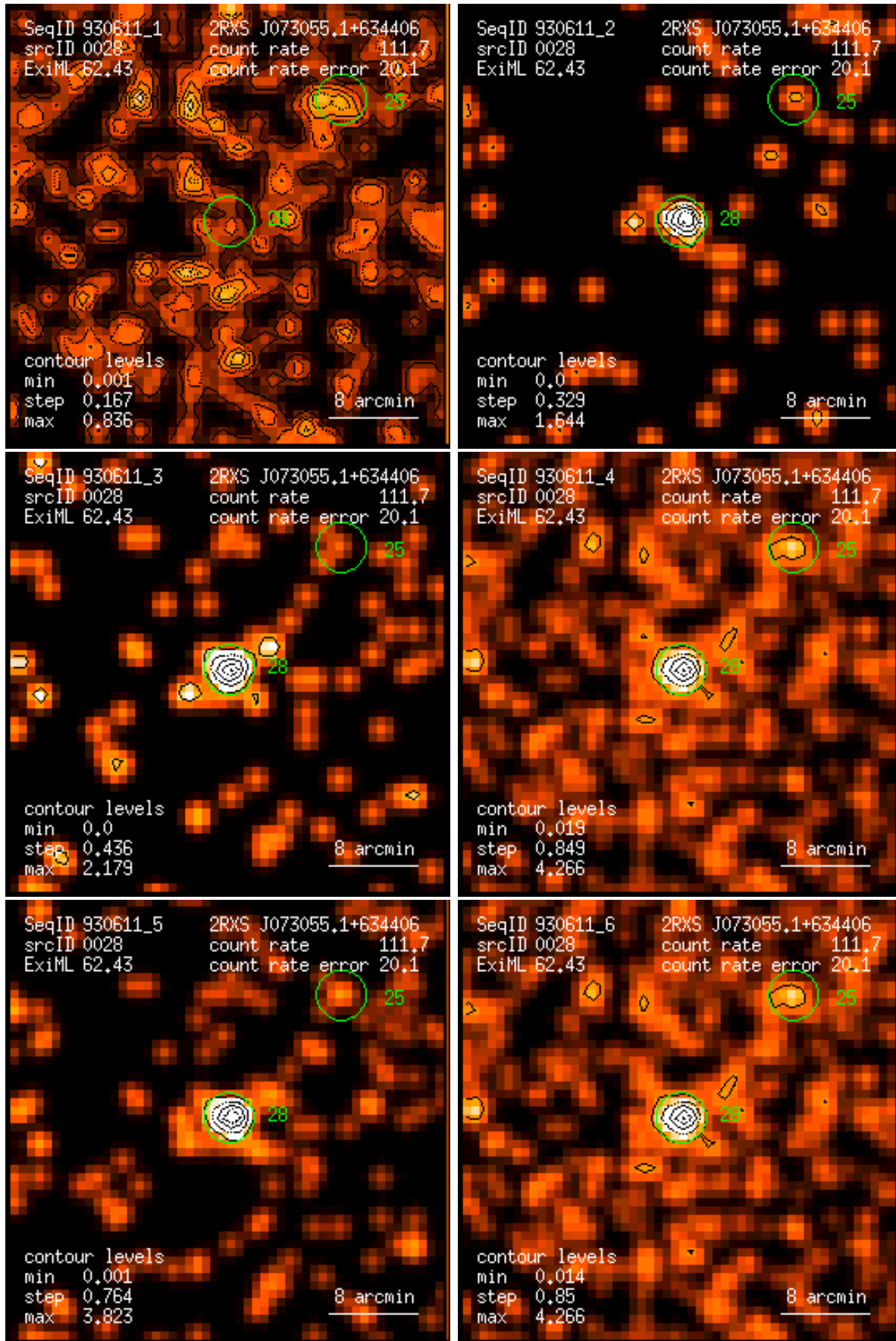
Figure 28: RASS 930611: detection 0028: band rate images, Gaussian filter: (1) PSPC channels 11 – 41, (2) 52 – 90, (3) 91 – 201, (4) 11 – 235, (5) 52 – 201, (6) 11 – 201. Broad band rates in counts/ks. Band rate contour levels in counts/ks/arcmin 2 .
