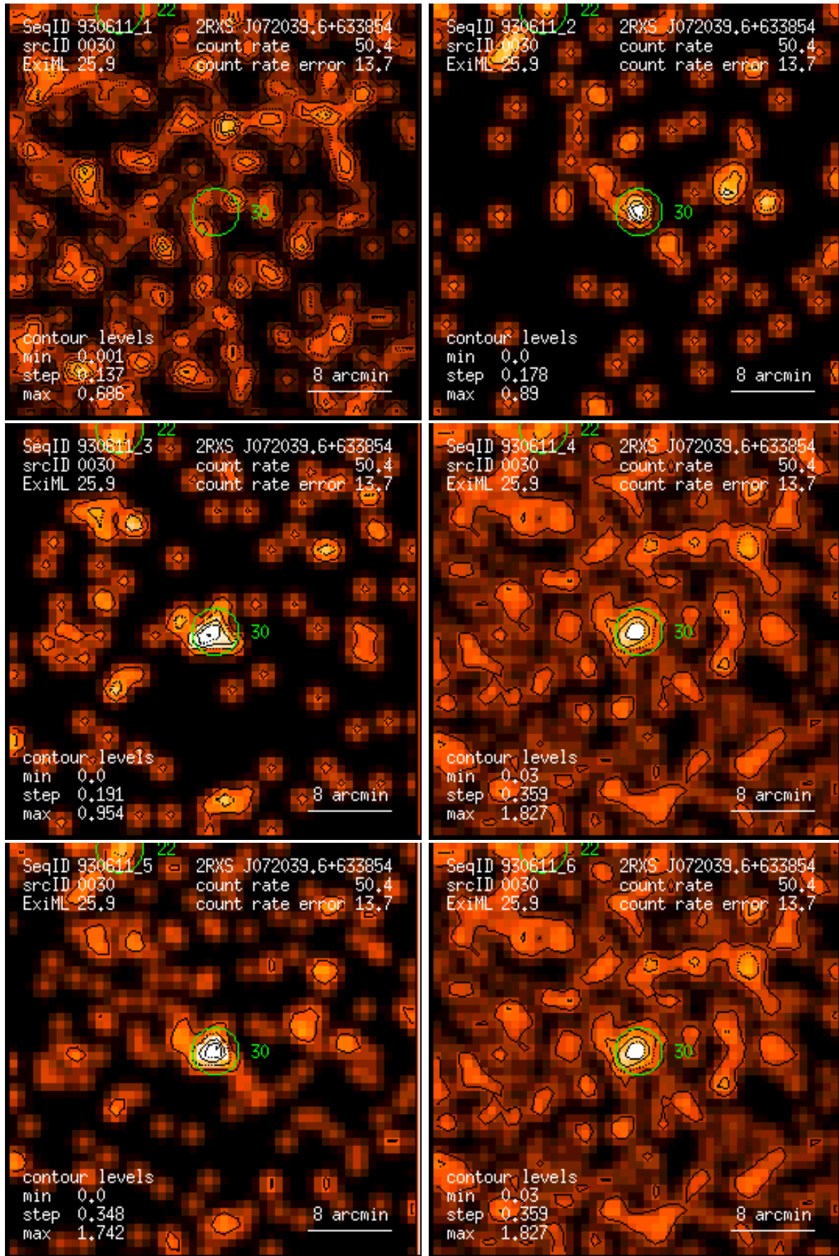
Figure 30: RASS 930611: detection 0030: band rate images, Gaussian filter: (1) PSPC channels 11 – 41, (2) 52 – 90, (3) 91 – 201, (4) 11 – 235, (5) 52 – 201, (6) 11 – 201. Broad band rates in counts/ks. Band rate contour levels in counts/ks/arcmin 2 .
