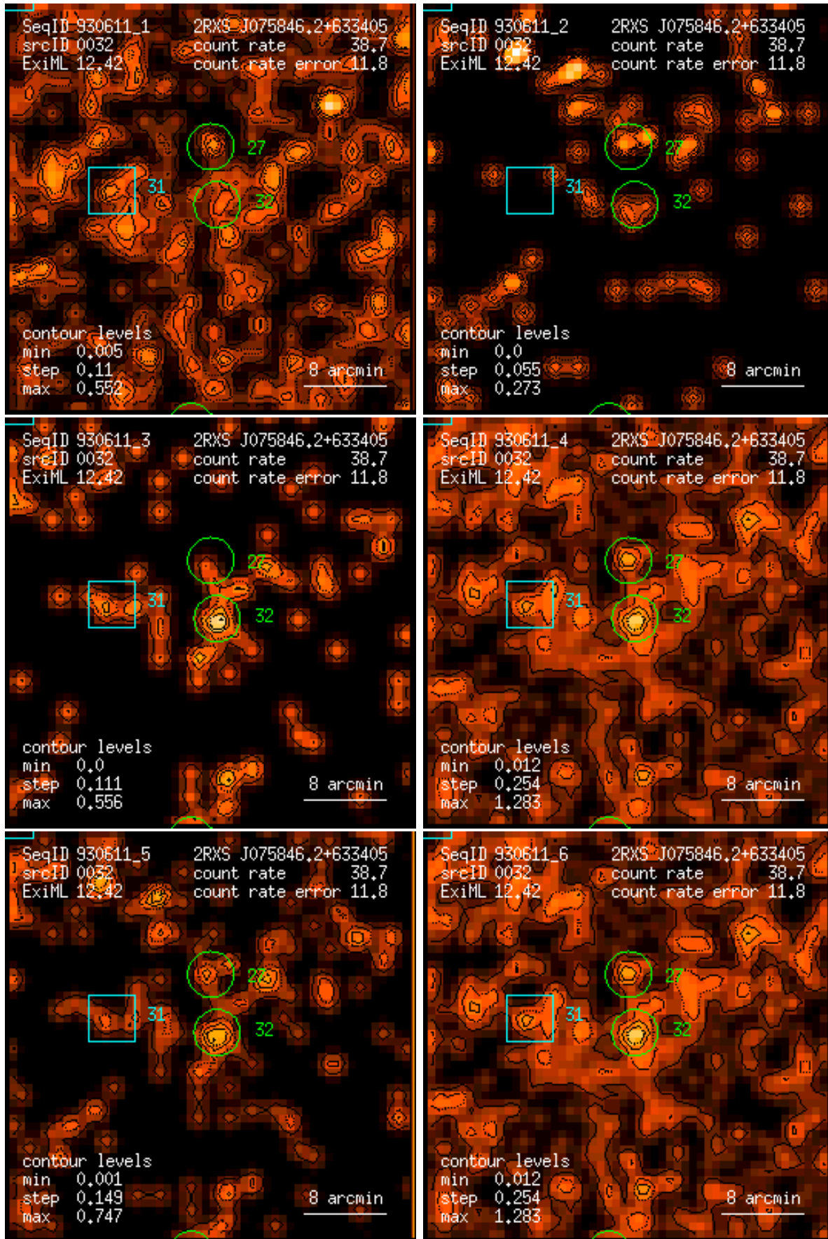
Figure 32: RASS 930611: detection 0032: band rate images, Gaussian filter: (1) PSPC channels 11 – 41, (2) 52 – 90, (3) 91 – 201, (4) 11 – 235, (5) 52 – 201, (6) 11 – 201. Broad band rates in counts/ks. Band rate contour levels in counts/ks/arcmin 2 .
