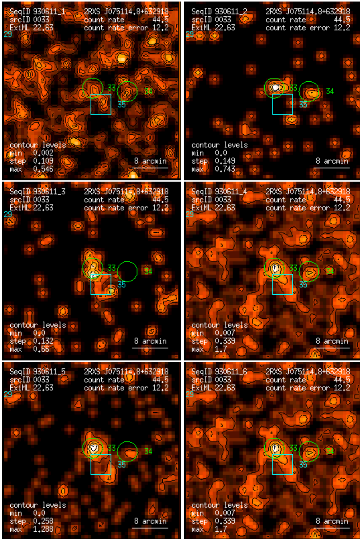
Figure 33: RASS 930611: detection 0033: band rate images, Gaussian filter: (1) PSPC channels 11 – 41, (2) 52 – 90, (3) 91 – 201, (4) 11 – 235, (5) 52 – 201, (6) 11 – 201. Broad band rates in counts/ks. Band rate contour levels in counts/ks/arcmin 2 .
