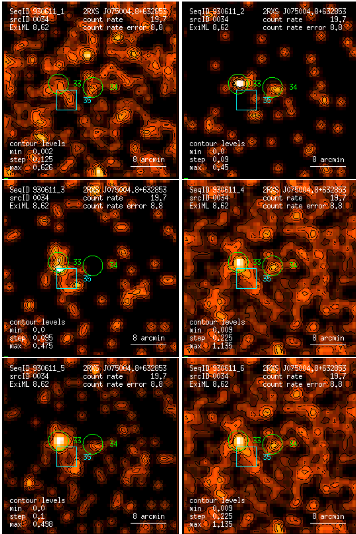
Figure 34: RASS 930611: detection 0034: band rate images, Gaussian filter: (1) PSPC channels 11 – 41, (2) 52 – 90, (3) 91 – 201, (4) 11 – 235, (5) 52 – 201, (6) 11 – 201. Broad band rates in counts/ks. Band rate contour levels in counts/ks/arcmin 2 .
