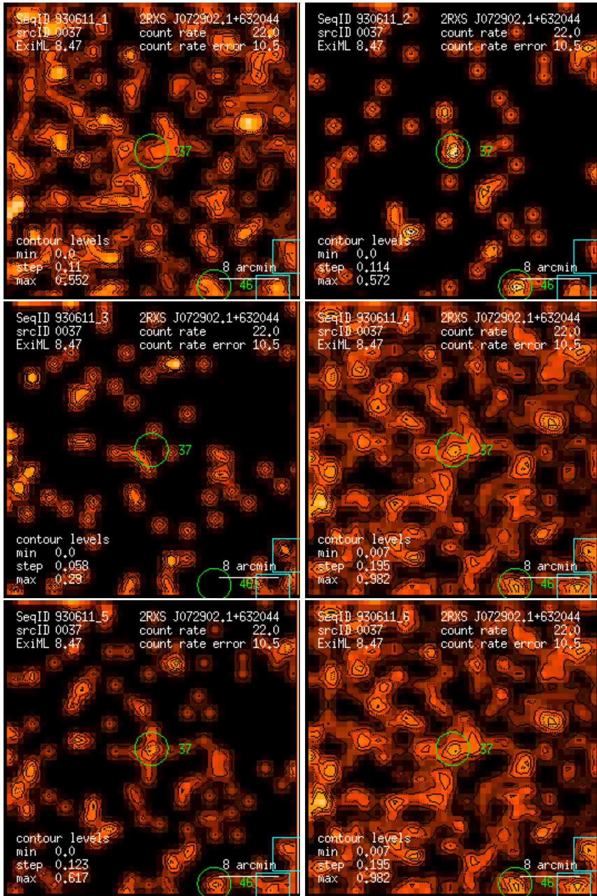
Figure 37: RASS 930611: detection 0037: band rate images, Gaussian filter: (1) PSPC channels 11 – 41, (2) 52 – 90, (3) 91 – 201, (4) 11 – 235, (5) 52 – 201, (6) 11 – 201. Broad band rates in counts/ks. Band rate contour levels in counts/ks/arcmin 2 .
