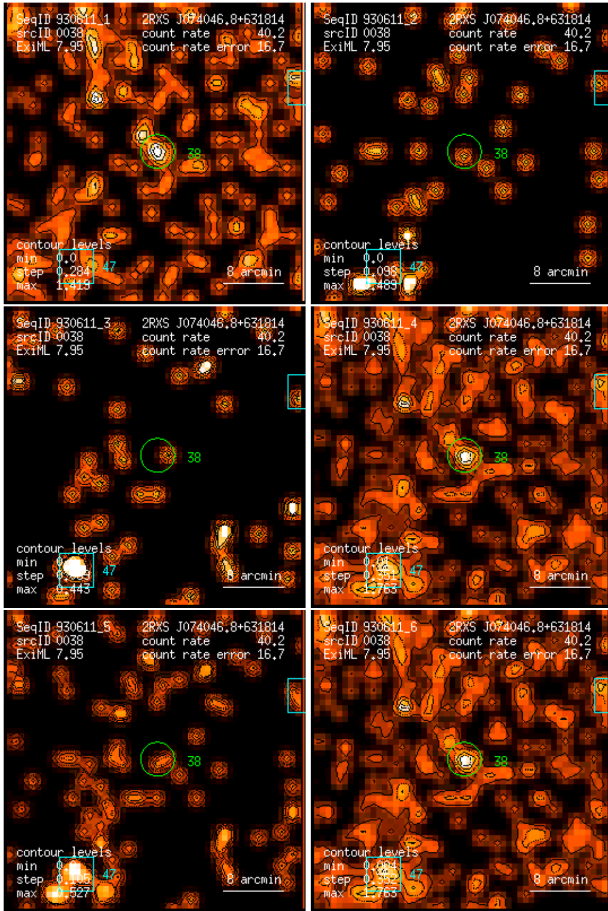
Figure 38: RASS 930611: detection 0038: band rate images, Gaussian filter: (1) PSPC channels 11 – 41, (2) 52 – 90, (3) 91 – 201, (4) 11 – 235, (5) 52 – 201, (6) 11 – 201. Broad band rates in counts/ks. Band rate contour levels in counts/ks/arcmin 2 .
