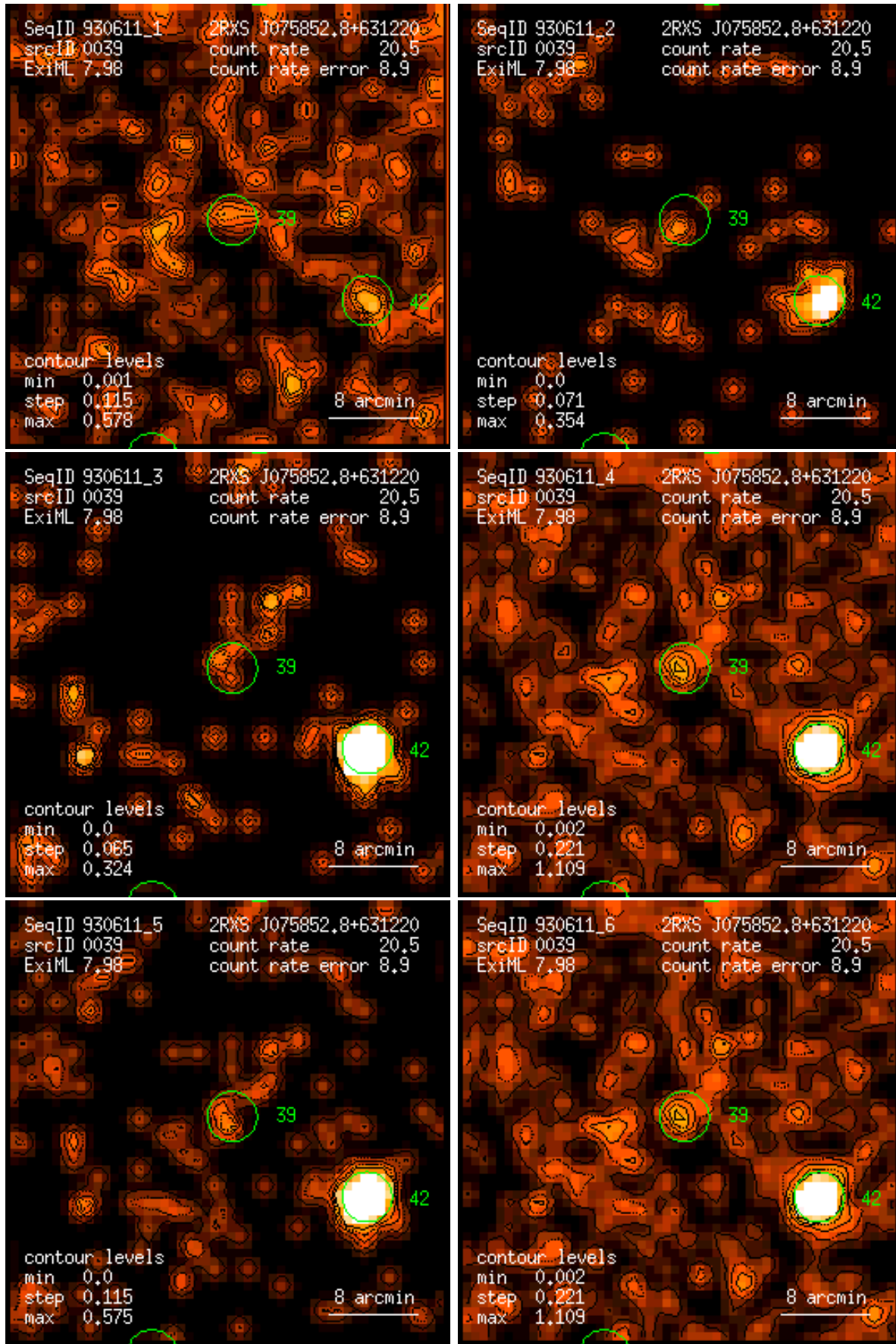
Figure 39: RASS 930611: detection 0039: band rate images, Gaussian filter: (1) PSPC channels 11 – 41, (2) 52 – 90, (3) 91 – 201, (4) 11 – 235, (5) 52 – 201, (6) 11 – 201. Broad band rates in counts/ks. Band rate contour levels in counts/ks/arcmin 2 .
