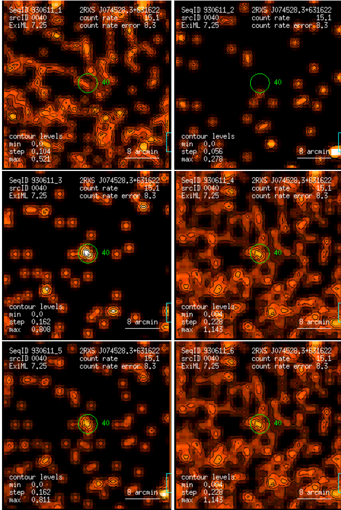
Figure 40: RASS 930611: detection 0040: band rate images, Gaussian filter: (1) PSPC channels 11 – 41, (2) 52 – 90, (3) 91 – 201, (4) 11 – 235, (5) 52 – 201, (6) 11 – 201. Broad band rates in counts/ks. Band rate contour levels in counts/ks/arcmin 2 .
