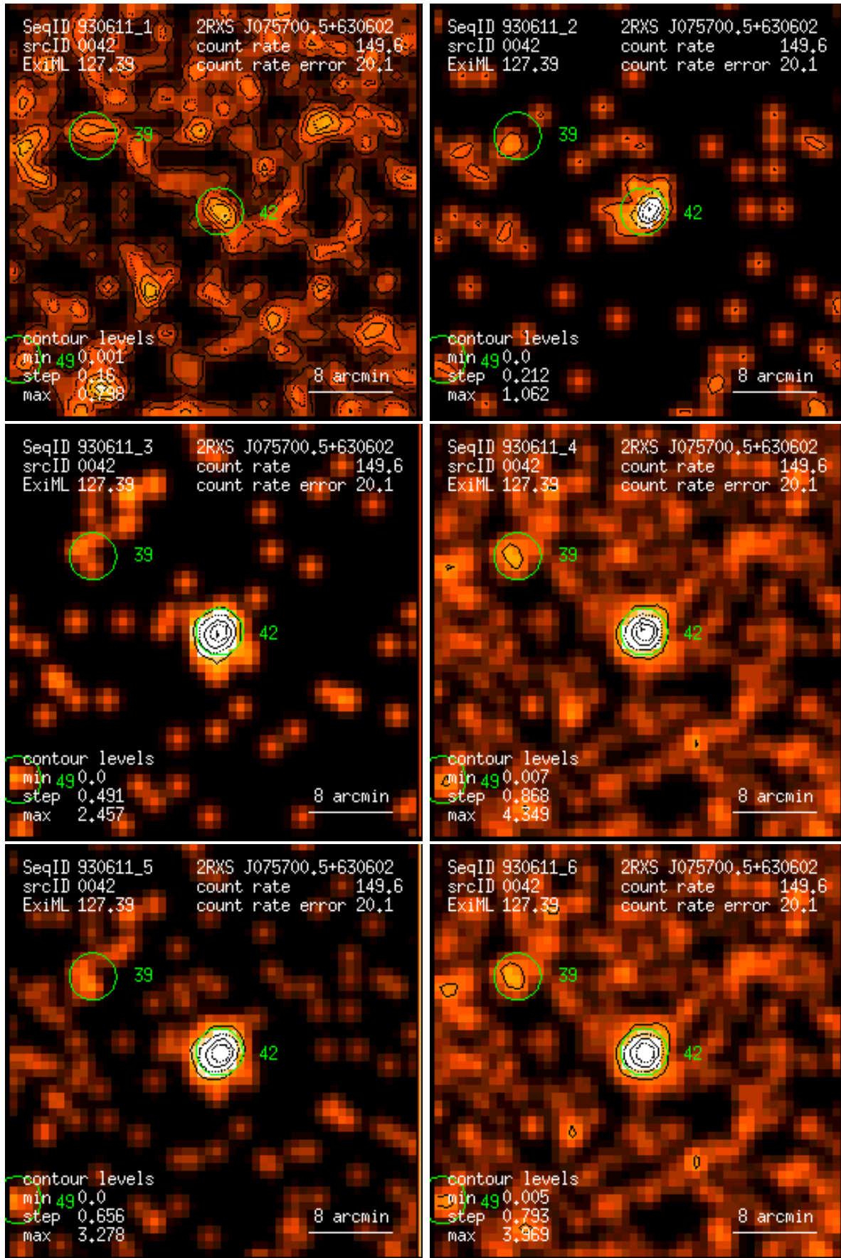
Figure 42: RASS 930611: detection 0042: band rate images, Gaussian filter: (1) PSPC channels 11 – 41, (2) 52 – 90, (3) 91 – 201, (4) 11 – 235, (5) 52 – 201, (6) 11 – 201. Broad band rates in counts/ks. Band rate contour levels in counts/ks/arcmin 2 .
