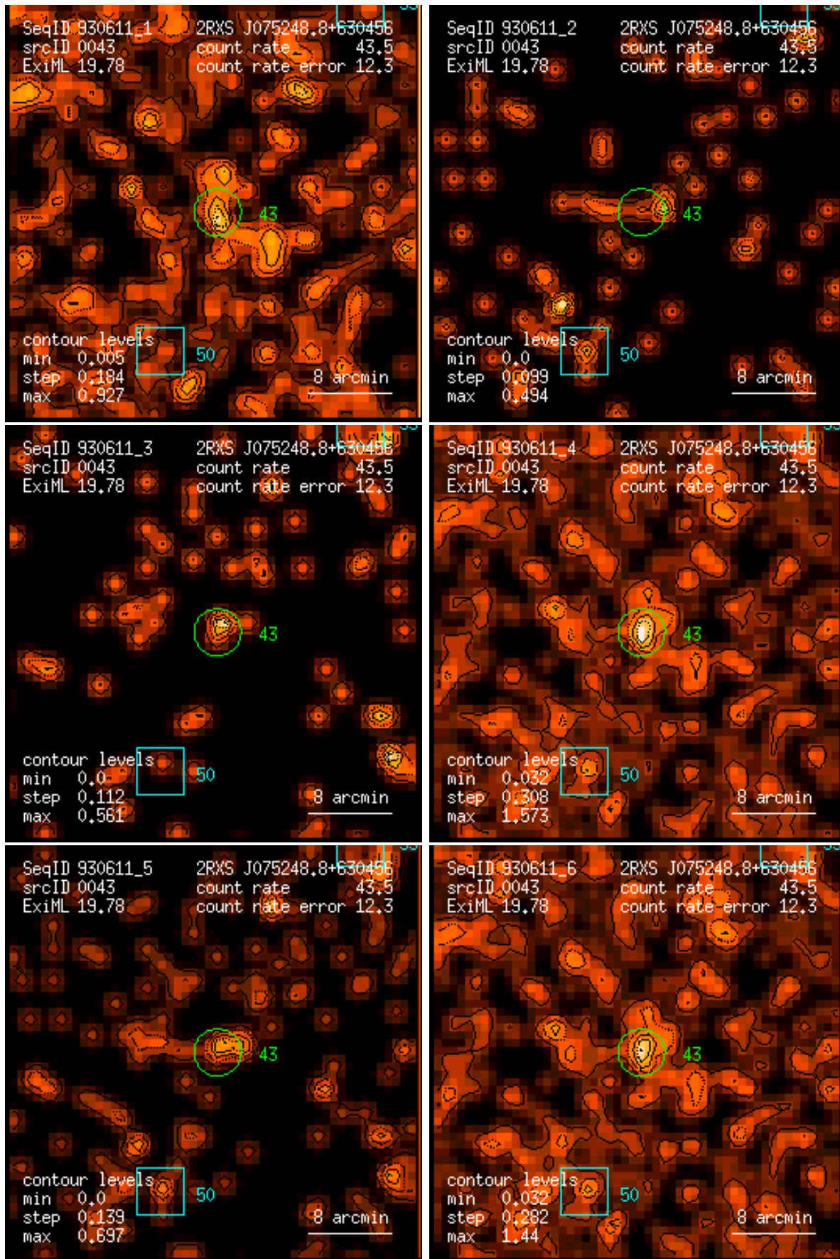
Figure 43: RASS 930611: detection 0043: band rate images, Gaussian filter: (1) PSPC channels 11 – 41, (2) 52 – 90, (3) 91 – 201, (4) 11 – 235, (5) 52 – 201, (6) 11 – 201. Broad band rates in counts/ks. Band rate contour levels in counts/ks/arcmin 2 .
