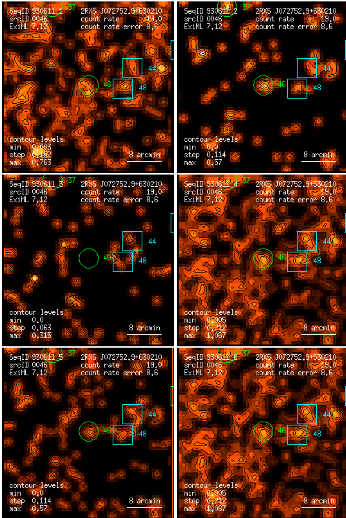
Figure 46: RASS 930611: detection 0046: band rate images, Gaussian filter: (1) PSPC channels 11 – 41, (2) 52 – 90, (3) 91 – 201, (4) 11 – 235, (5) 52 – 201, (6) 11 – 201. Broad band rates in counts/ks. Band rate contour levels in counts/ks/arcmin 2 .
