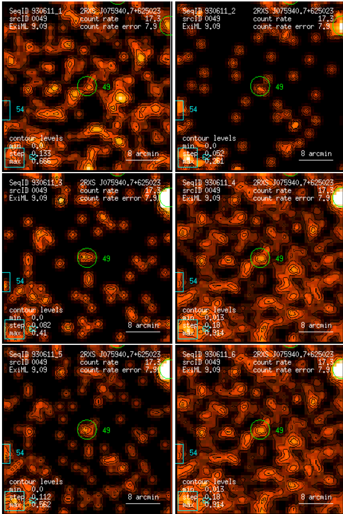
Figure 49: RASS 930611: detection 0049: band rate images, Gaussian filter: (1) PSPC channels 11 – 41, (2) 52 – 90, (3) 91 – 201, (4) 11 – 235, (5) 52 – 201, (6) 11 – 201. Broad band rates in counts/ks. Band rate contour levels in counts/ks/arcmin 2 .
