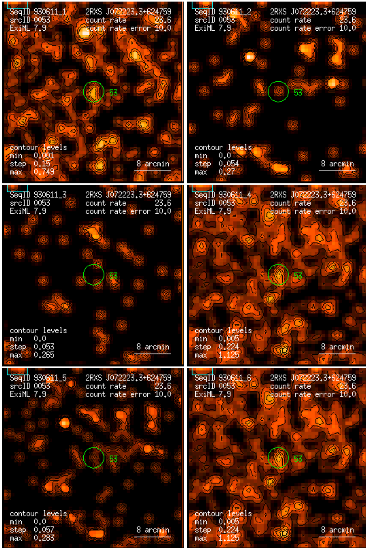
Figure 53: RASS 930611: detection 0053: band rate images, Gaussian filter: (1) PSPC channels 11 – 41, (2) 52 – 90, (3) 91 – 201, (4) 11 – 235, (5) 52 – 201, (6) 11 – 201. Broad band rates in counts/ks. Band rate contour levels in counts/ks/arcmin 2 .
