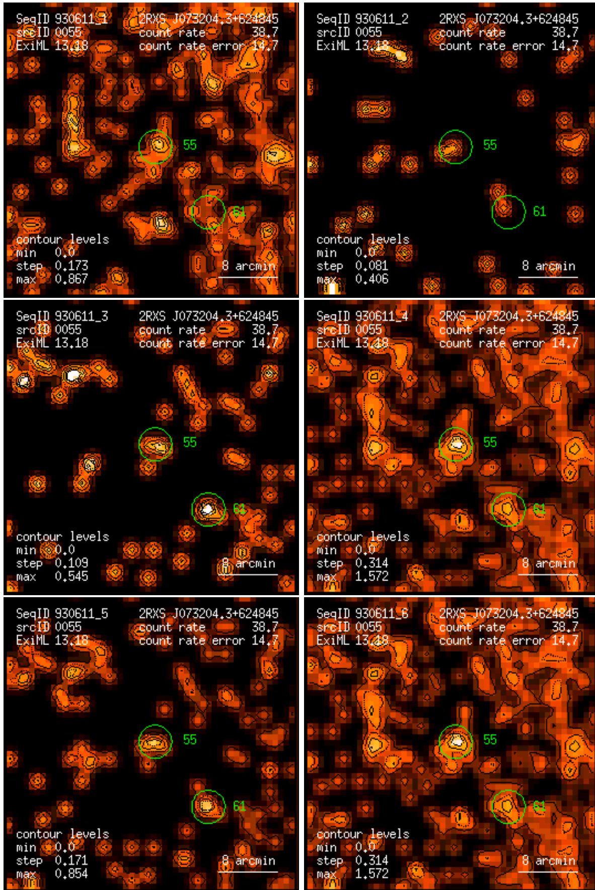
Figure 55: RASS 930611: detection 0055: band rate images, Gaussian filter: (1) PSPC channels 11 – 41, (2) 52 – 90, (3) 91 – 201, (4) 11 – 235, (5) 52 – 201, (6) 11 – 201. Broad band rates in counts/ks. Band rate contour levels in counts/ks/arcmin 2 .
