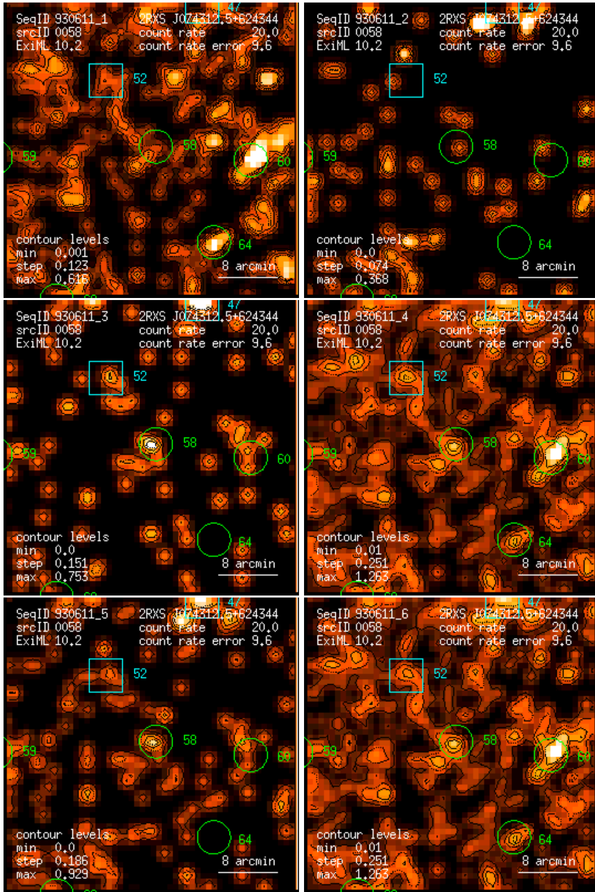
Figure 58: RASS 930611: detection 0058: band rate images, Gaussian filter: (1) PSPC channels 11 – 41, (2) 52 – 90, (3) 91 – 201, (4) 11 – 235, (5) 52 – 201, (6) 11 – 201. Broad band rates in counts/ks. Band rate contour levels in counts/ks/arcmin 2 .
