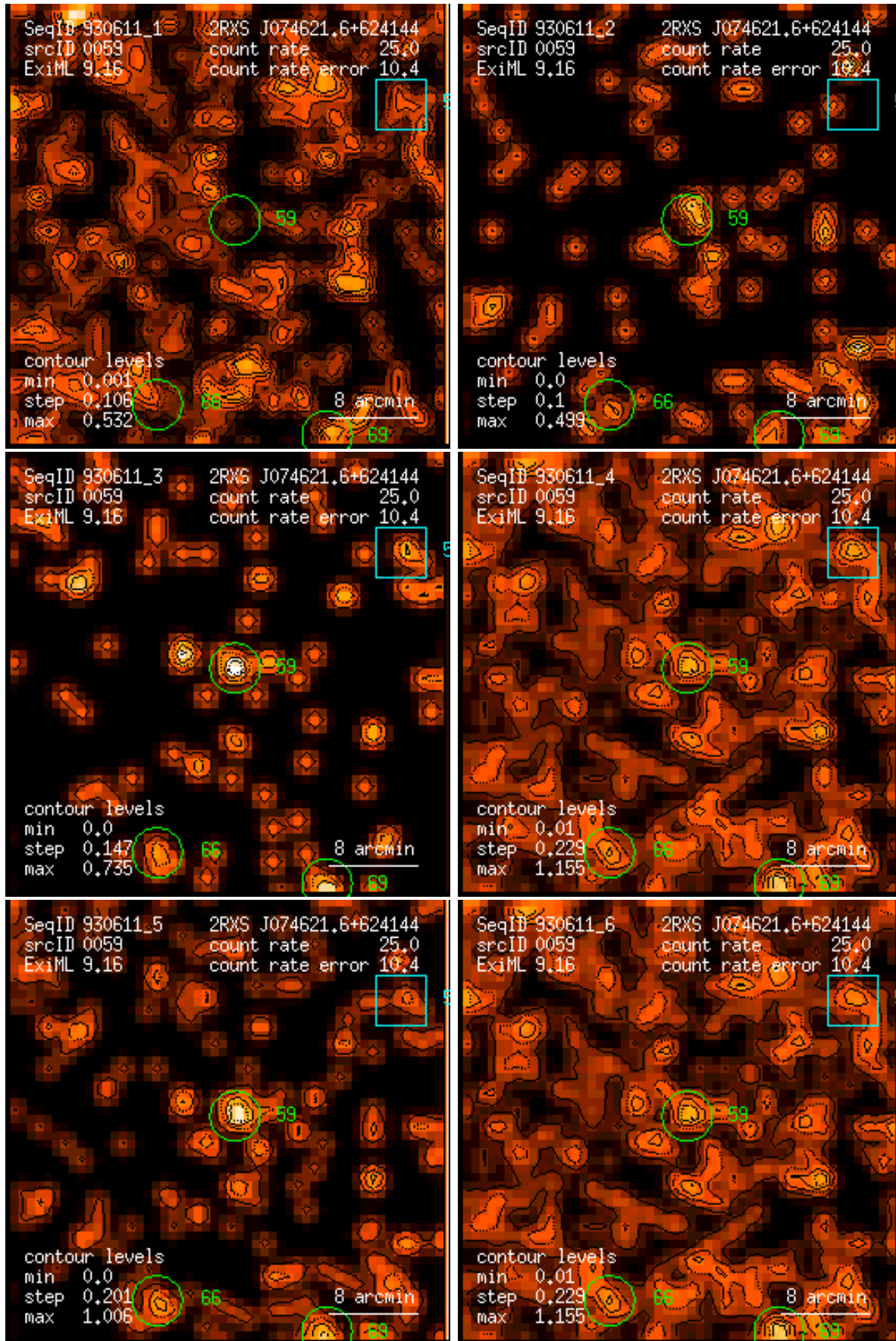
Figure 59: RASS 930611: detection 0059: band rate images, Gaussian filter: (1) PSPC channels 11 – 41, (2) 52 – 90, (3) 91 – 201, (4) 11 – 235, (5) 52 – 201, (6) 11 – 201. Broad band rates in counts/ks. Band rate contour levels in counts/ks/arcmin 2 .
