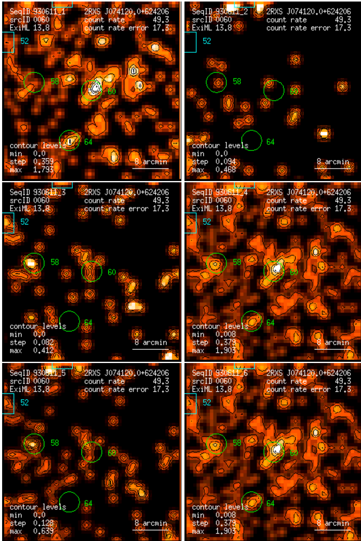
Figure 60: RASS 930611: detection 0060: band rate images, Gaussian filter: (1) PSPC channels 11 – 41, (2) 52 – 90, (3) 91 – 201, (4) 11 – 235, (5) 52 – 201, (6) 11 – 201. Broad band rates in counts/ks. Band rate contour levels in counts/ks/arcmin 2 .
