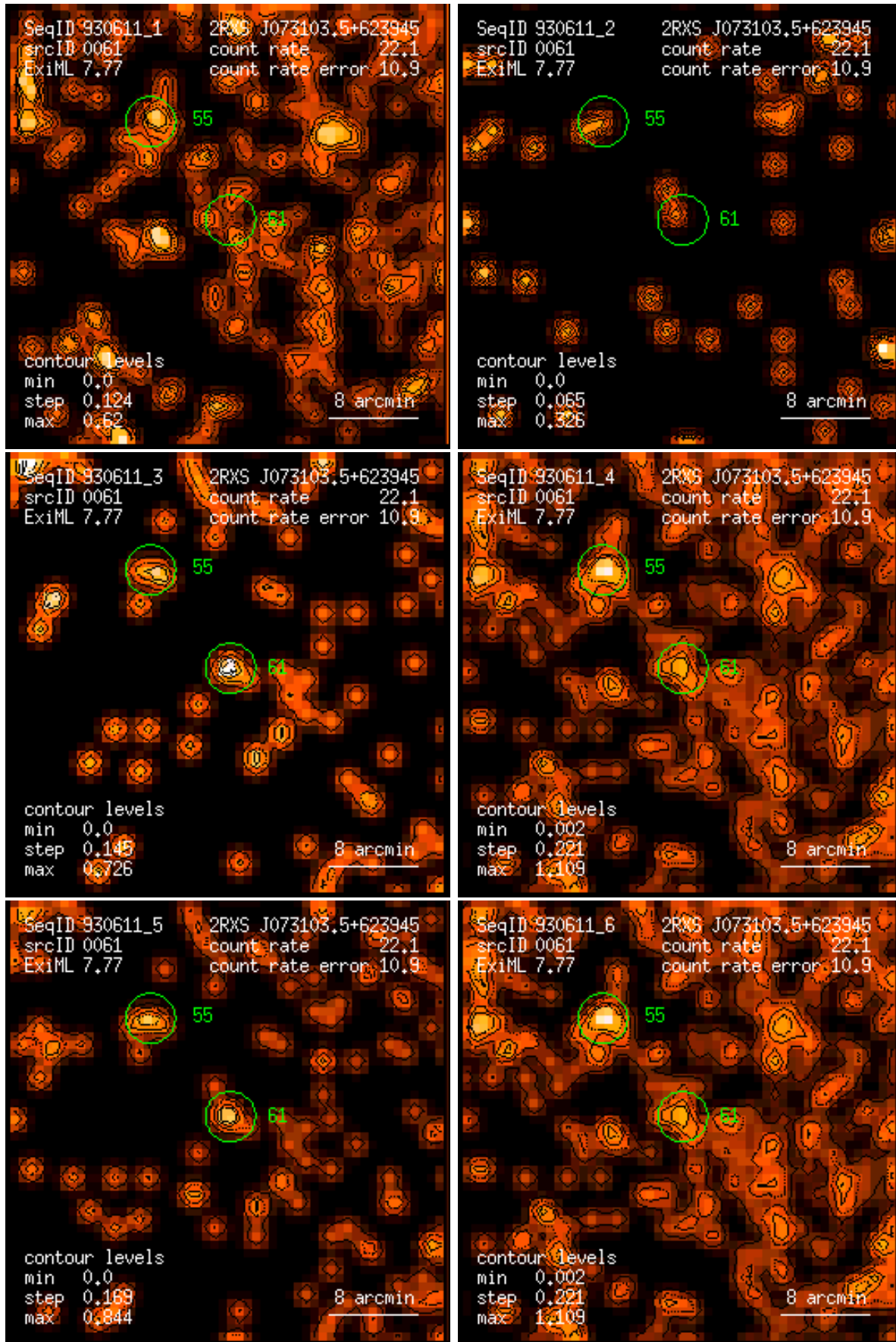
Figure 61: RASS 930611: detection 0061: band rate images, Gaussian filter: (1) PSPC channels 11 – 41, (2) 52 – 90, (3) 91 – 201, (4) 11 – 235, (5) 52 – 201, (6) 11 – 201. Broad band rates in counts/ks. Band rate contour levels in counts/ks/arcmin 2 .
