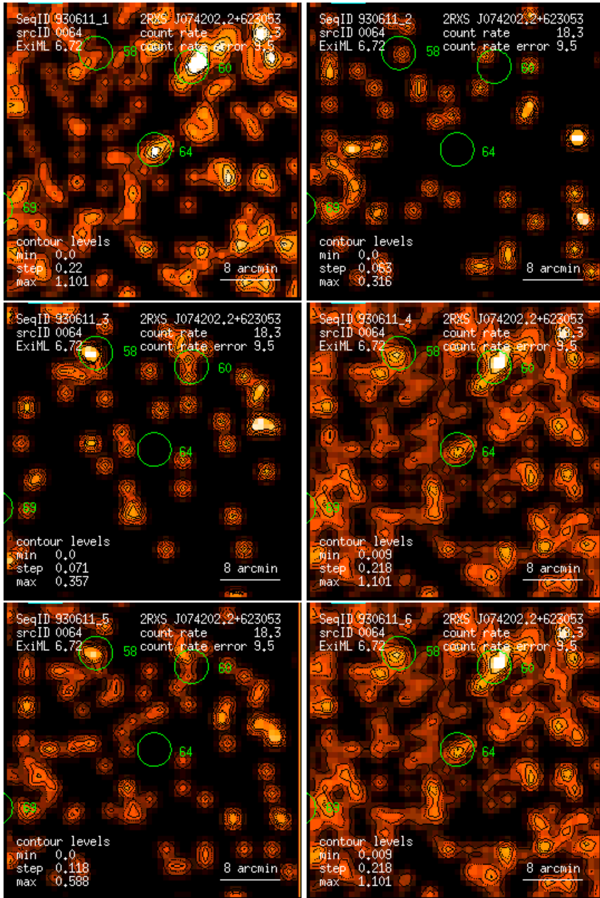
Figure 64: RASS 930611: detection 0064: band rate images, Gaussian filter: (1) PSPC channels 11 – 41, (2) 52 – 90, (3) 91 – 201, (4) 11 – 235, (5) 52 – 201, (6) 11 – 201. Broad band rates in counts/ks. Band rate contour levels in counts/ks/arcmin 2 .
