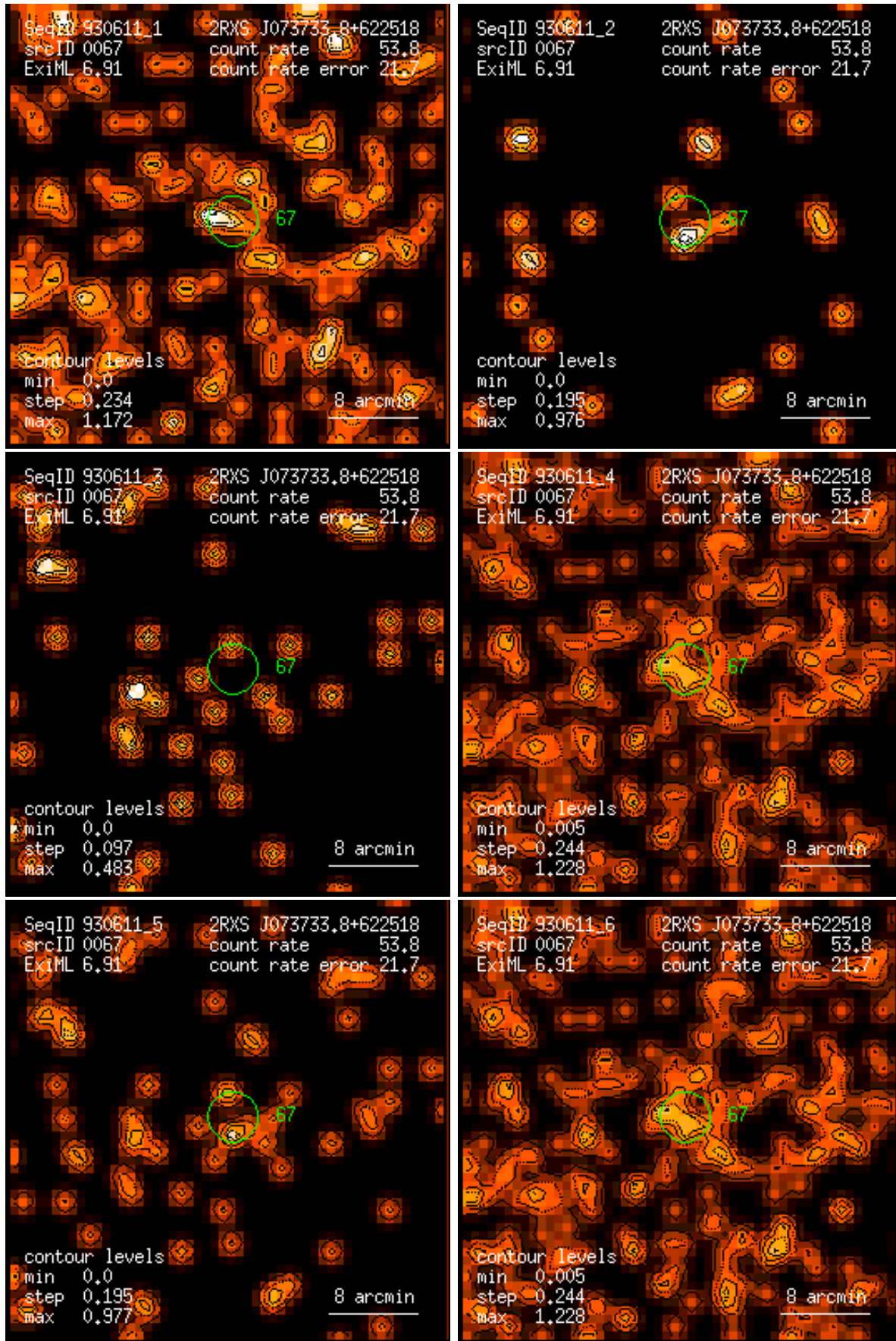
Figure 67: RASS 930611: detection 0067: band rate images, Gaussian filter: (1) PSPC channels 11 – 41, (2) 52 – 90, (3) 91 – 201, (4) 11 – 235, (5) 52 – 201, (6) 11 – 201. Broad band rates in counts/ks. Band rate contour levels in counts/ks/arcmin 2 .
