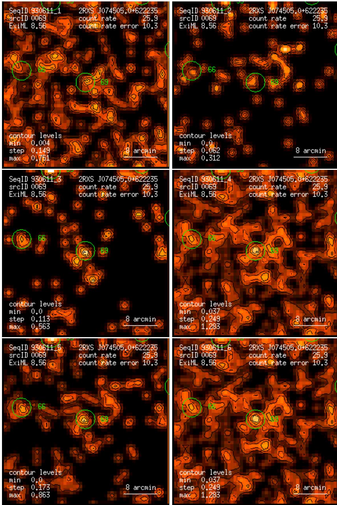
Figure 69: RASS 930611: detection 0069: band rate images, Gaussian filter: (1) PSPC channels 11 – 41, (2) 52 – 90, (3) 91 – 201, (4) 11 – 235, (5) 52 – 201, (6) 11 – 201. Broad band rates in counts/ks. Band rate contour levels in counts/ks/arcmin 2 .
