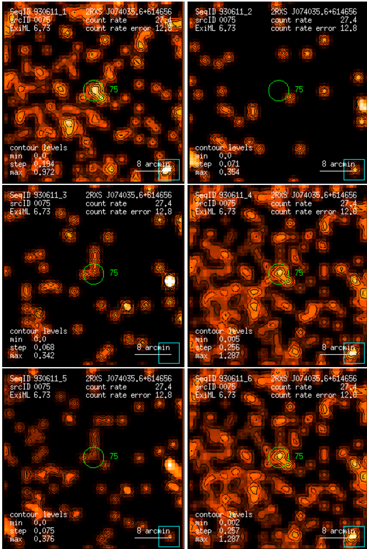
Figure 75: RASS 930611: detection 0075: band rate images, Gaussian filter: (1) PSPC channels 11 – 41, (2) 52 – 90, (3) 91 – 201, (4) 11 – 235, (5) 52 – 201, (6) 11 – 201. Broad band rates in counts/ks. Band rate contour levels in counts/ks/arcmin 2 .
