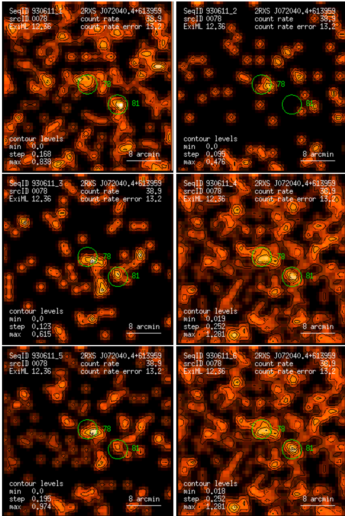
Figure 78: RASS 930611: detection 0078: band rate images, Gaussian filter: (1) PSPC channels 11 – 41, (2) 52 – 90, (3) 91 – 201, (4) 11 – 235, (5) 52 – 201, (6) 11 – 201. Broad band rates in counts/ks. Band rate contour levels in counts/ks/arcmin 2 .
