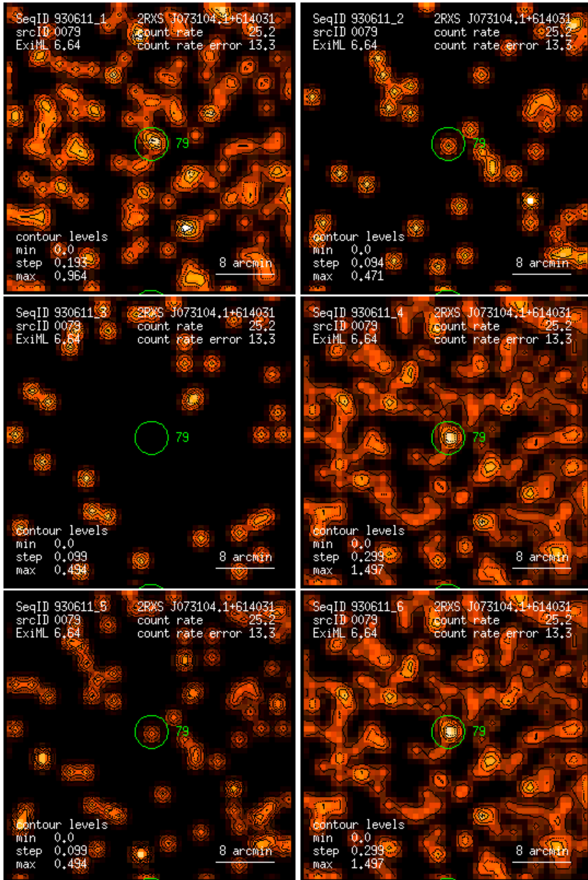
Figure 79: RASS 930611: detection 0079: band rate images, Gaussian filter: (1) PSPC channels 11 – 41, (2) 52 – 90, (3) 91 – 201, (4) 11 – 235, (5) 52 – 201, (6) 11 – 201. Broad band rates in counts/ks. Band rate contour levels in counts/ks/arcmin 2 .
