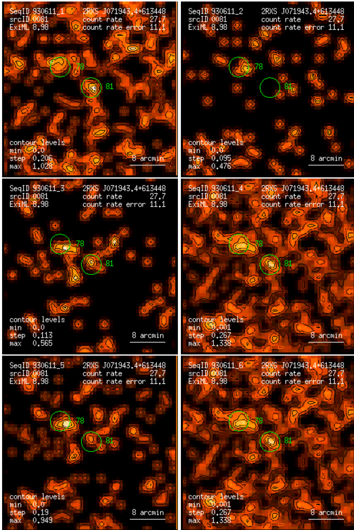
Figure 81: RASS 930611: detection 0081: band rate images, Gaussian filter: (1) PSPC channels 11 – 41, (2) 52 – 90, (3) 91 – 201, (4) 11 – 235, (5) 52 – 201, (6) 11 – 201. Broad band rates in counts/ks. Band rate contour levels in counts/ks/arcmin 2 .
