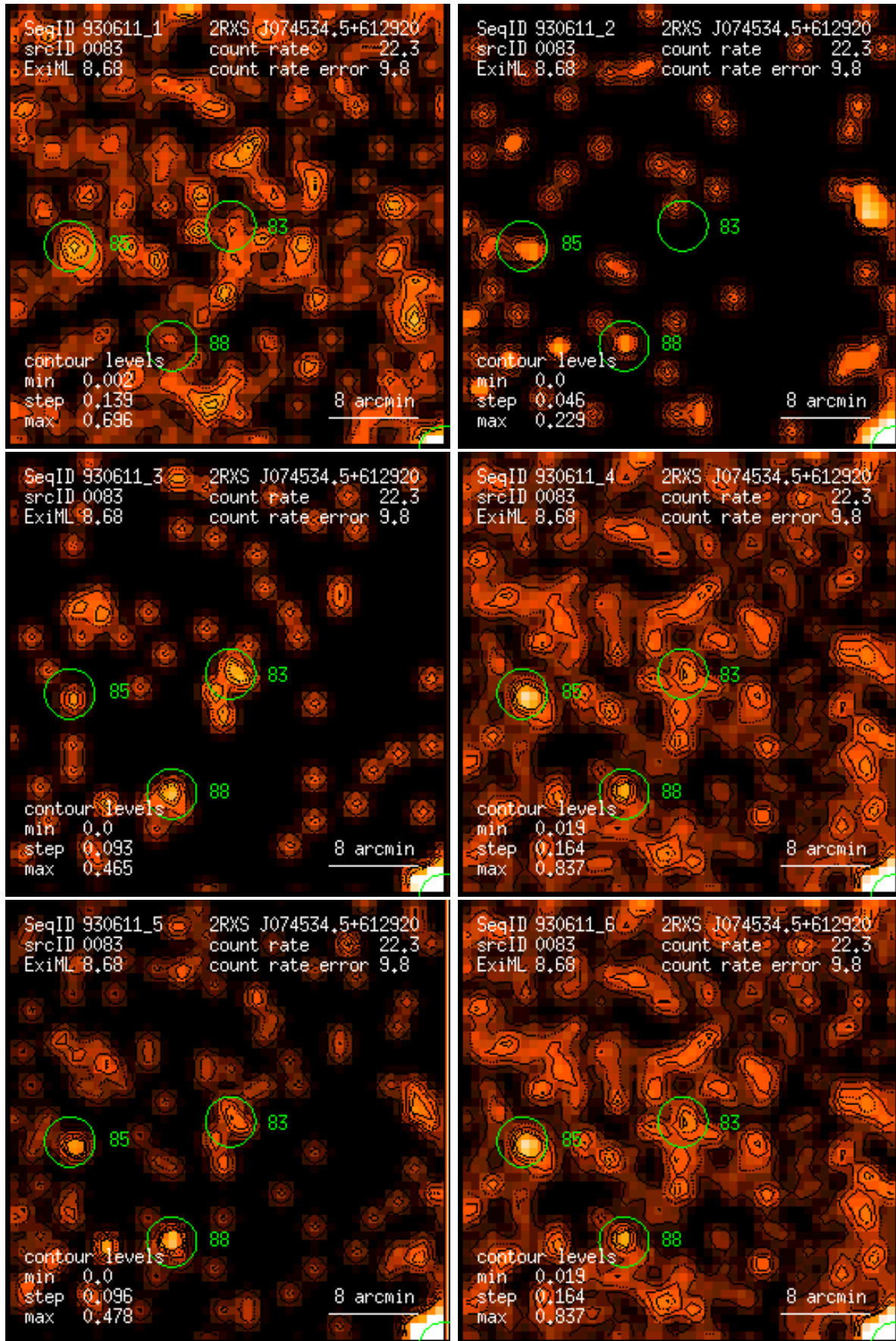
Figure 83: RASS 930611: detection 0083: band rate images, Gaussian filter: (1) PSPC channels 11 – 41, (2) 52 – 90, (3) 91 – 201, (4) 11 – 235, (5) 52 – 201, (6) 11 – 201. Broad band rates in counts/ks. Band rate contour levels in counts/ks/arcmin 2 .
