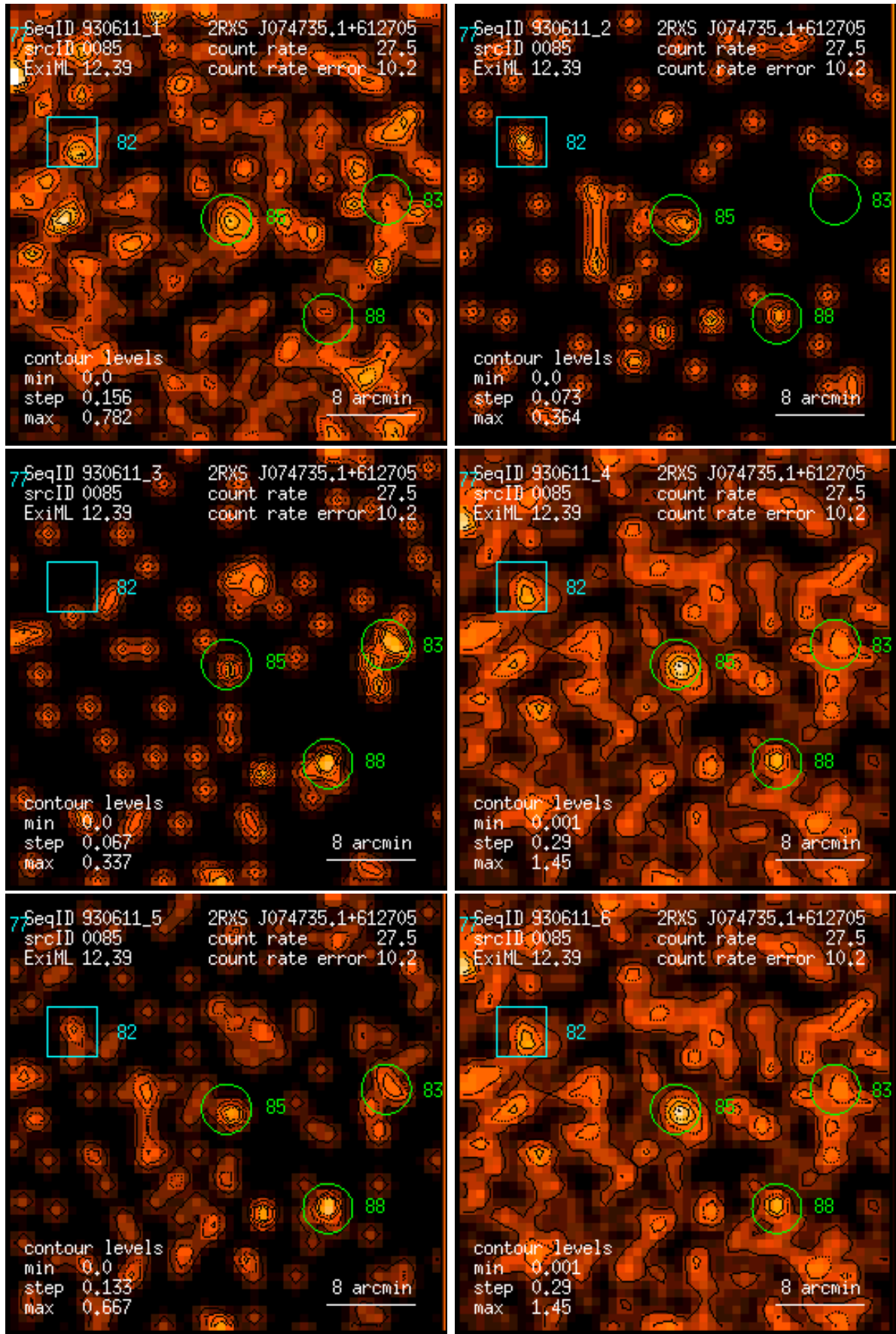
Figure 85: RASS 930611: detection 0085: band rate images, Gaussian filter: (1) PSPC channels 11 – 41, (2) 52 – 90, (3) 91 – 201, (4) 11 – 235, (5) 52 – 201, (6) 11 – 201. Broad band rates in counts/ks. Band rate contour levels in counts/ks/arcmin 2 .
