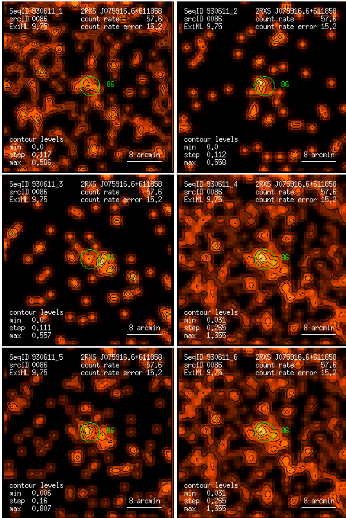
Figure 86: RASS 930611: detection 0086: band rate images, Gaussian filter: (1) PSPC channels 11 – 41, (2) 52 – 90, (3) 91 – 201, (4) 11 – 235, (5) 52 – 201, (6) 11 – 201. Broad band rates in counts/ks. Band rate contour levels in counts/ks/arcmin 2 .
