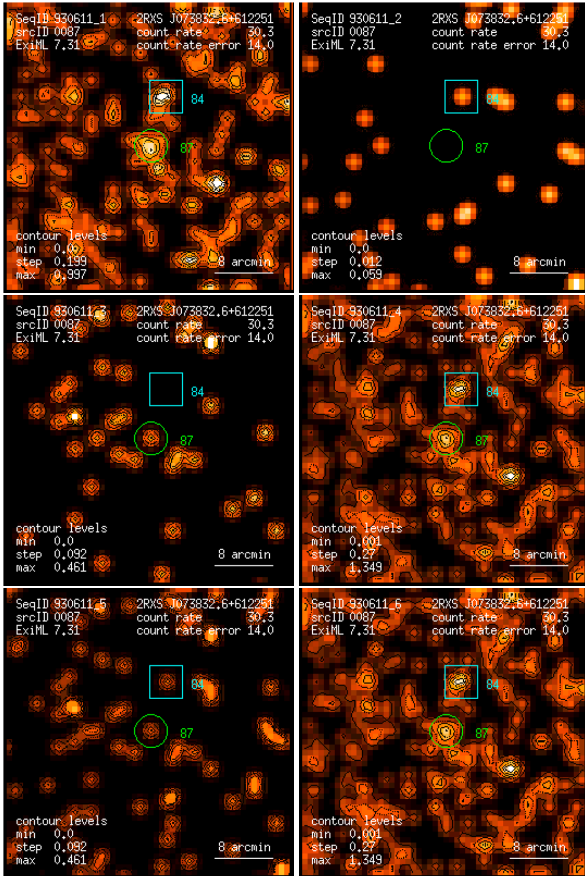
Figure 87: RASS 930611: detection 0087: band rate images, Gaussian filter: (1) PSPC channels 11 – 41, (2) 52 – 90, (3) 91 – 201, (4) 11 – 235, (5) 52 – 201, (6) 11 – 201. Broad band rates in counts/ks. Band rate contour levels in counts/ks/arcmin 2 .
