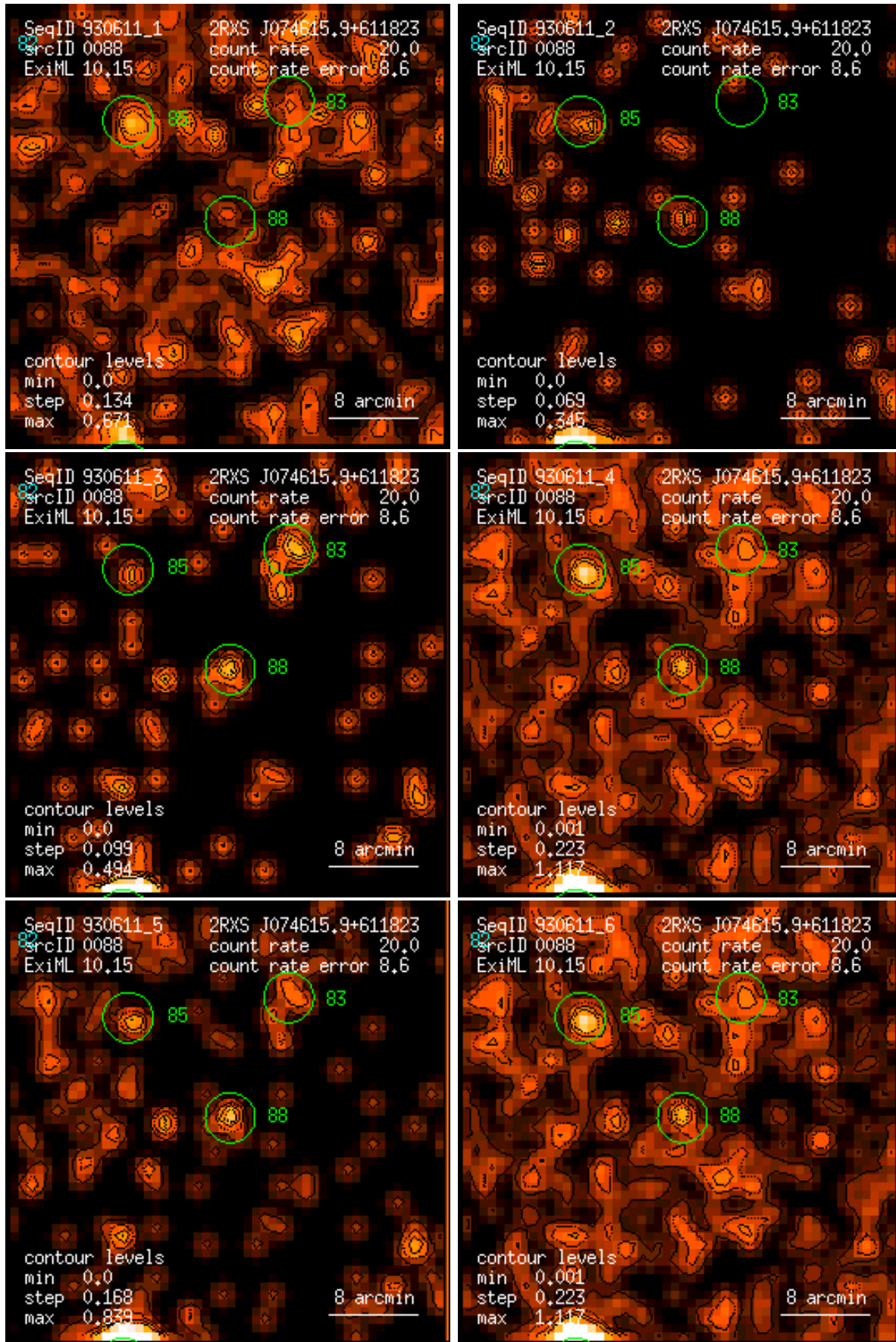
Figure 88: RASS 930611: detection 0088: band rate images, Gaussian filter: (1) PSPC channels 11 – 41, (2) 52 – 90, (3) 91 – 201, (4) 11 – 235, (5) 52 – 201, (6) 11 – 201. Broad band rates in counts/ks. Band rate contour levels in counts/ks/arcmin 2 .
