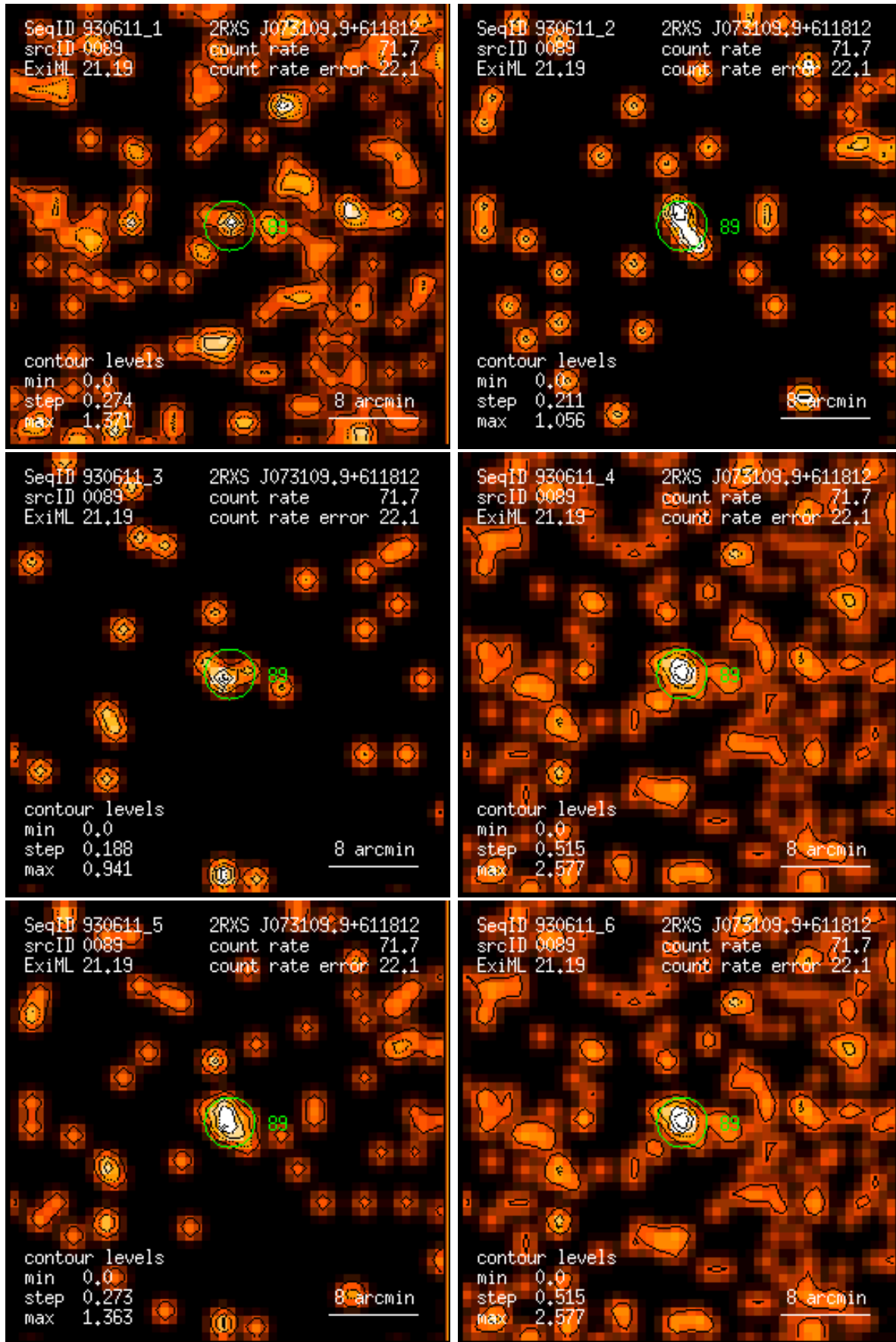
Figure 89: RASS 930611: detection 0089: band rate images, Gaussian filter: (1) PSPC channels 11 – 41, (2) 52 – 90, (3) 91 – 201, (4) 11 – 235, (5) 52 – 201, (6) 11 – 201. Broad band rates in counts/ks. Band rate contour levels in counts/ks/arcmin 2 .
